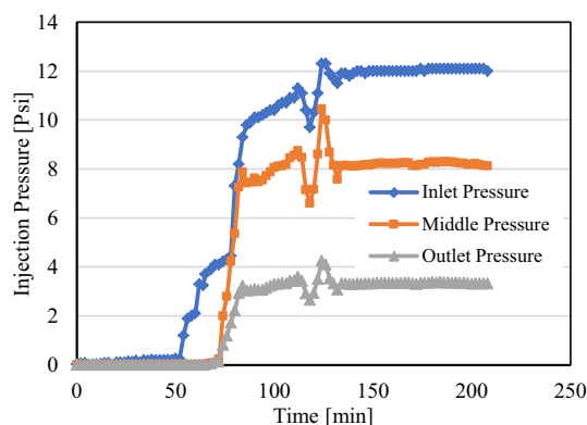
Fig. 9 Gel propagation injection pressure through fractures 6.75 mm using 1450 pa strength (gel particle size to fracture width ratio is 0.47)
