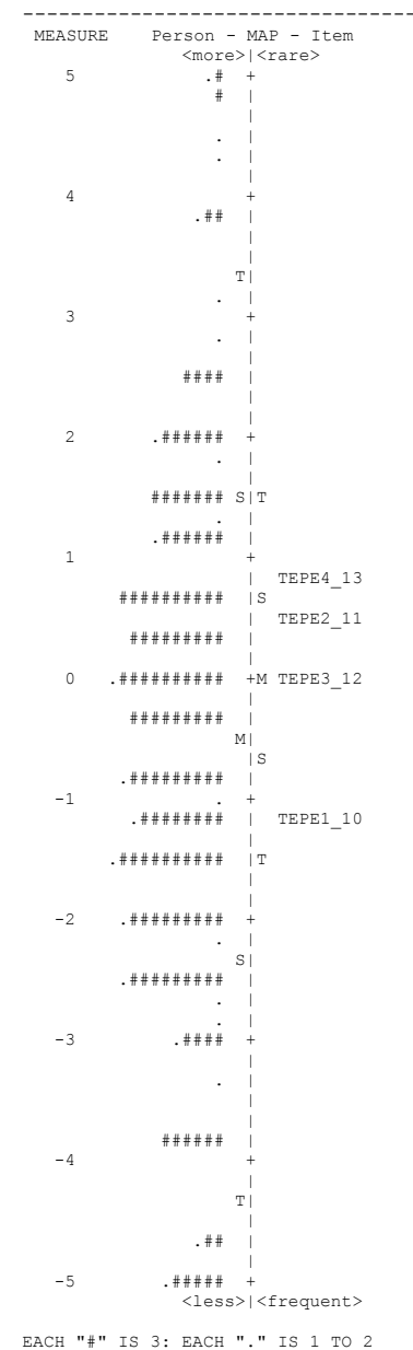
Figure 2. Item-person map of external political efficacy
