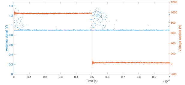
Fig. 6. PD activity detection by means of a horn antenna, simultaneously with the detection of Fig. 4.
