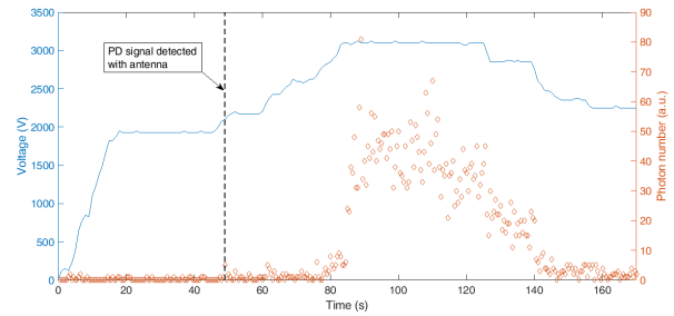
Fig. 7. PD activity detection in a motor by means of the optic sensor, using 50 Hz AC voltage. The latter is expressed in peak-to-peak.
