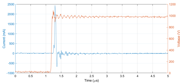
Fig. 5. PD activity measurement by means of a Hall effect current probe, simultaneously with the detection of Fig. 4. The identification is possible using a technique such as that described in the work of Borghi et al [13].
