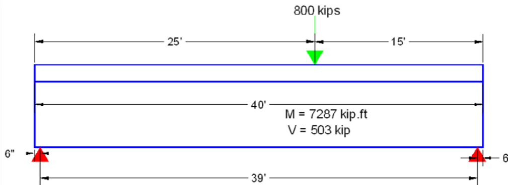
Figure 13. Girder (B) test setup
