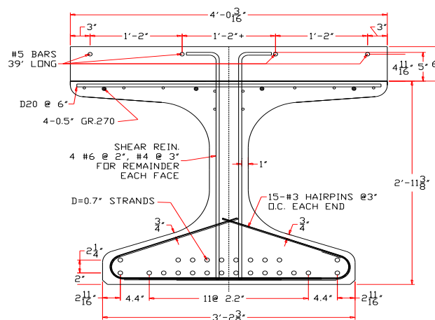
Figure 7. NU900 girder (Pacific Street Project, Omaha, NE) [3]
