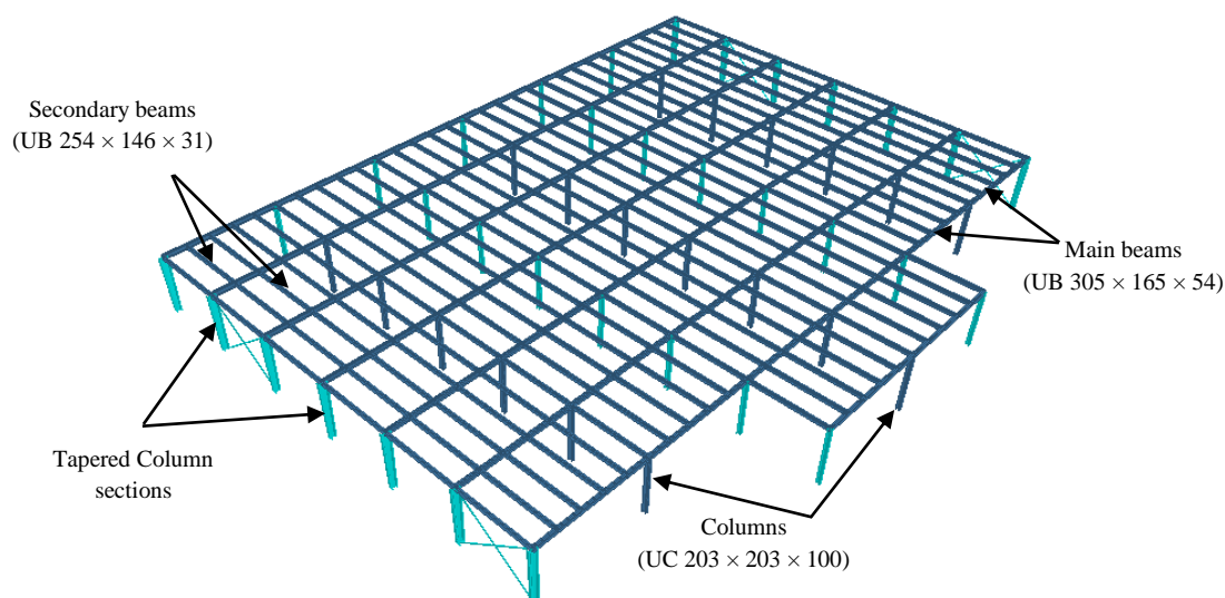
Figure 4. Isomeric 3D rendered view of the mezzanine floor
