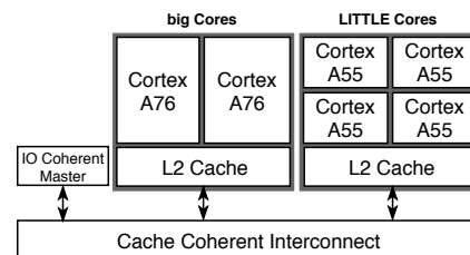
Fig. 3: Example of an ARM big.LITTLE architecture.
