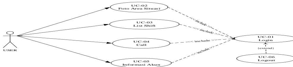
Gambar 3 Use Case Diagram
