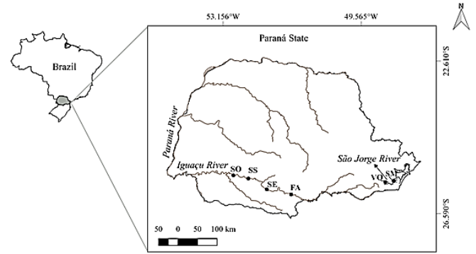
Figure 2. Location of the six Neotropical reservoirs sampled from January 2005 to December 2007. SO=Salto Osório, SS=Salto Santiago, SE=Segredo, FA=Foz do Areia, VO=Vossoroca and SM=Salto do Meio.
