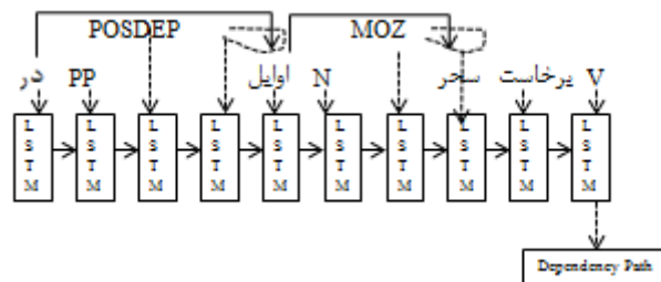
Figure 4. An example of dependency path feature extraction using LSTM network of pair of predicate and its candidate argument (برخاست، در) from sentence shown in Figure 2-b.
