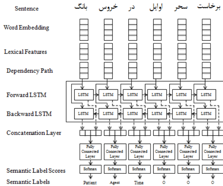
Figure 3. An example of Persian SRL using our proposed model.
