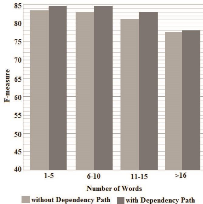
Figure 6. Results on second corpus by sentence length.
