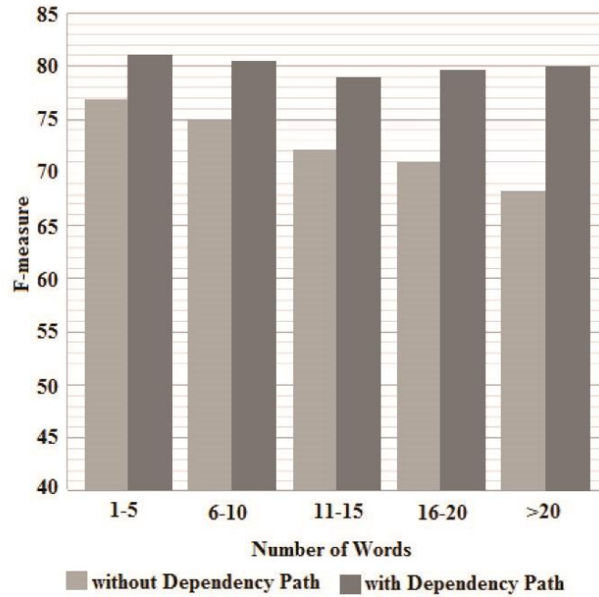
Figure 5. Results on first corpus by sentence length.
