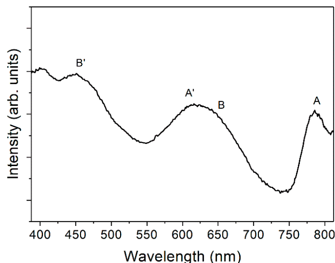
Figure 6. UV–VIS spectrum of WSe 2 .
