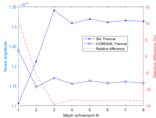
Figure 4.7 Effect of the spatial grid resolution on the amplitude of the thermal neutron noise at the location of the noise source
