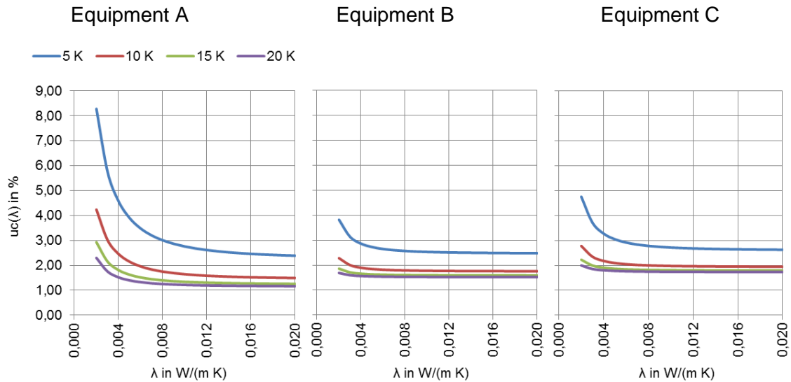
Figure 112: Combined relative uncertainty as a function of thermal conductivity for a panel thickness of 10mm for the example equipment A, B and C according to EN 1946-3:1999 with varying temperature difference.
