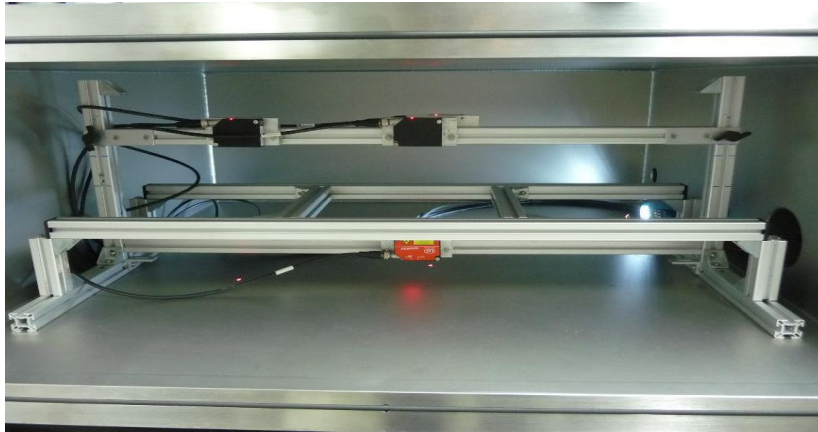
Figure 26: Equipment for determination of internal pressure measurement using the foil lift-off method in a vacuum chamber, laser measurement gauges are placed inside the vacuum chamber, VIPs are placed on a rectangular support with 250mm side length. Source: FIW München.
