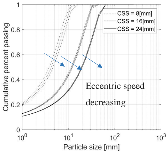
Figure 5. Product PSD of different cone crusher settings. Data from Evertsson (Evertsson, 2000), tested on a Svedala Hydrocone cone crusher.
