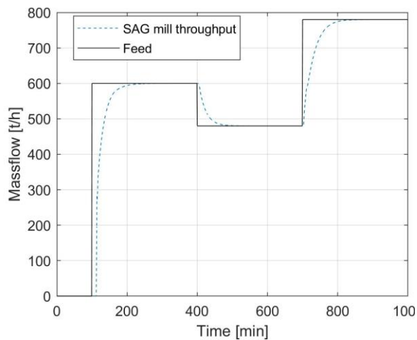
Figure 10. Dynamic response of the mill with a different feed rate.
