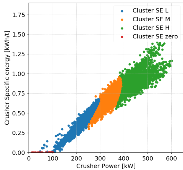
Figure 16. Clusters of recycling load based on crusher power and pebble specific energy.
