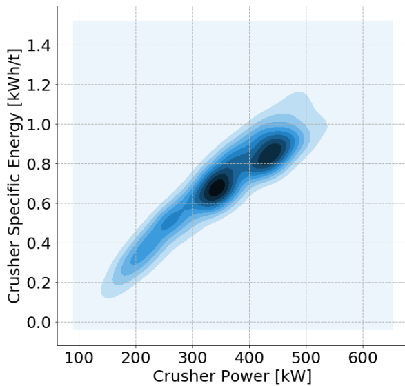
Figure 15. Kernel density estimation plot of the pebble crusher power and pebble specific energy.
