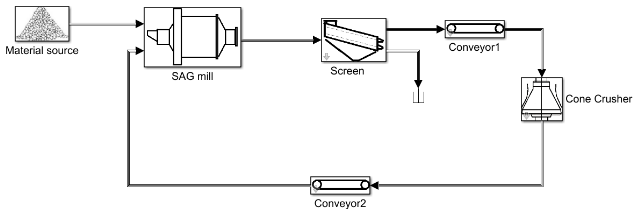
Figure 20. Flowsheet of the simulation scenario 1
