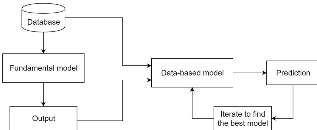
Figure 3. Schematic illustration of a hybrid fundamental-data model. The output of a physics-based model is used as a new feature in a data-based model, modified from Karpatne (Karpatne et al., 2017a).
