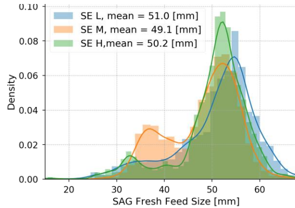
Figure 18 (b). The SAG mill feed size f_{80} distribution.
