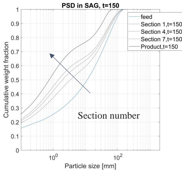
Figure 22. PSD in SAG mill, simulation time at 150 min
