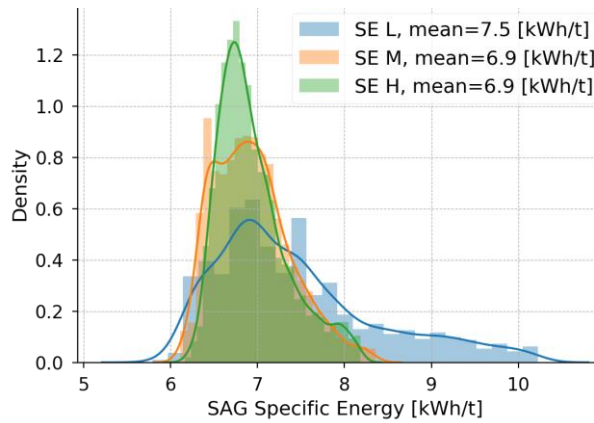
Figure 18 (a). The SAG mill specific energy distribution.
