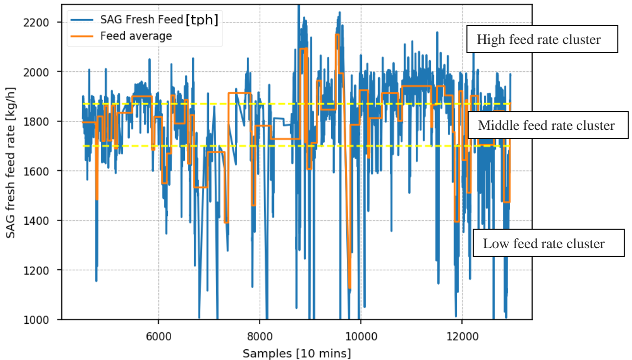
Figure 17. Change points of fresh feed rate. It is categorized into three classes based on their average value in each period.
