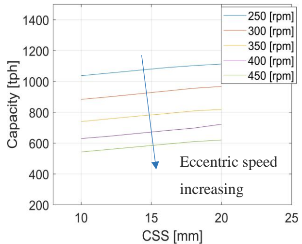
Figure 6. The capacity of cone crushers with different settings. Data from Lindqvist (Lindqvist and Evertsson, 2004), tested on an FLS Raptor 900 cone crusher.
