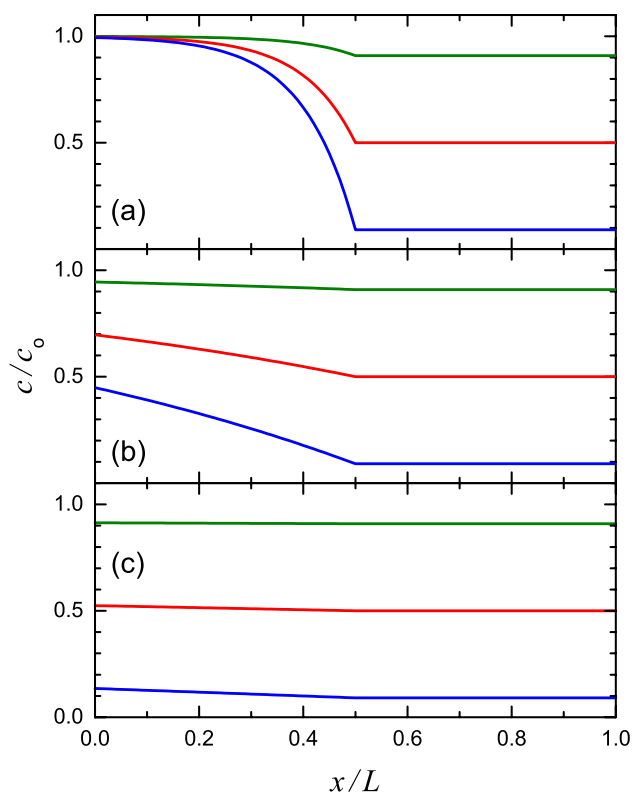
Fig. 4 Normalized reactant concentration along the nanochannel according to the model with the Danckwerts boundary conditions: a slow diffusion with D/vL = 0.1 , b moderate diffusion with D/vL = 1 , and c rapid diffusion with D/vL = 10 . In each cases, the results of calculations are shown for slow reaction with w_0/v = 0.1 (upper thick line), reaction with w_0/v = 1 (medium thick line), and rapid reaction with w_0/v = 10 (lower thick line). A catalytic nanoparticle is located in the center of the channel ( x_p = L/2 ). Note that with increasing diffusion coefficient or reaction rate constant the concentration becomes appreciably smaller than c_0 even near the channel inlet (at x = 0 )
