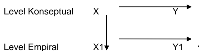
Diagram 1: Pengujian Hipotesis
