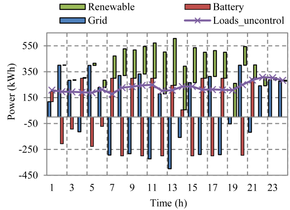
Fig. 9 Energy balance of the whole microgrid in the first scenario
