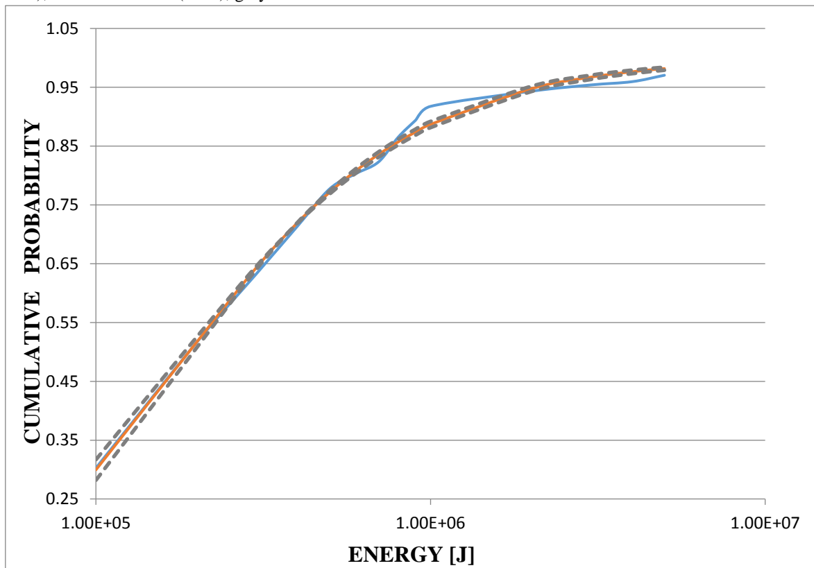
Fig.13. Seismic energy distribution curves for low-energy shocks from the Bytom syncline region (1987 – 2012). Blue – empirical (ECD), red – theoretical (CDF), greys – 5% confidence intervals for CDF
