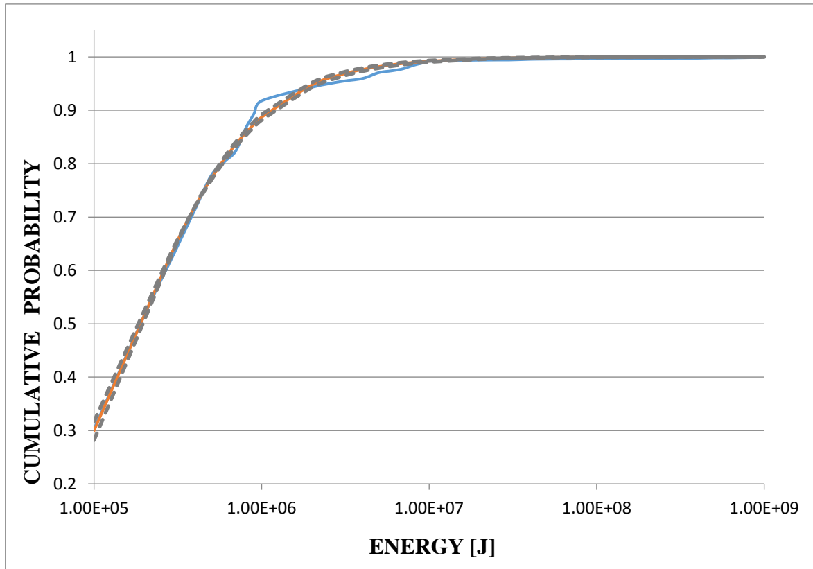
Fig.12. Seismic energy distribution curves from the Bytom syncline region (1987 – 2012). Blue – empirical (ECD), red – theoretical (CDF), greys – 5% confidence intervals for CDF
