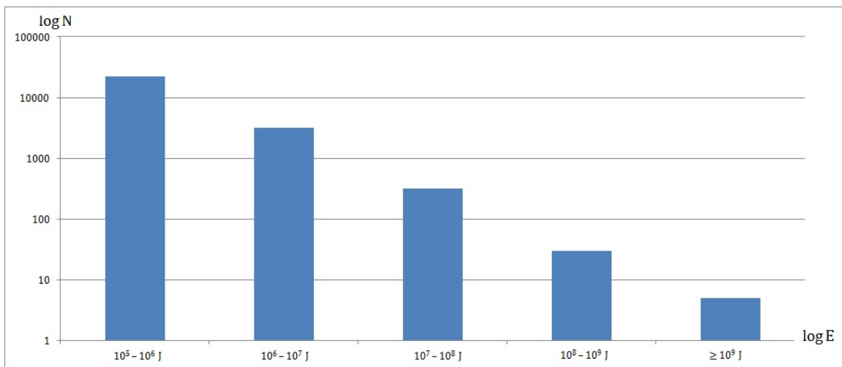
Fig.2. Histogram presenting logarithmic number of tremors for energy intervals 10^5 - 10^6 J (22607 tremors), 10^6 - 10^7 J (3160 tremors), 10^7 - 10^8 J (321 tremors), 10^8 - 10^9 J (30 tremors), E \geq 10^9 J (5 tremors) for the whole USCBB. N – number of events, E - energy
