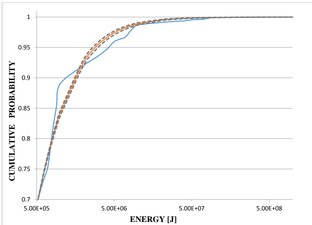
Fig.11. Seismic energy distribution curves for high-energy shocks from the main antycline region (1987 – 2012). Blue – empirical (ECD), red – theoretical (CDF), greys – 5% confidence intervals for CDF
