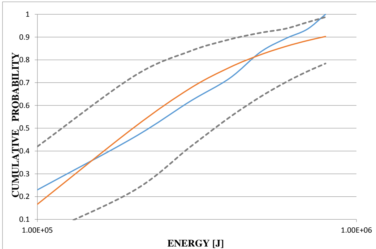
Fig.5. Seismic energy distribution curves for low-energy shocks from the main syncline region (1987 – 2012). Blue – empirical (ECD), red – theoretical (CDF), greys – 5% confidence intervals for CDF
