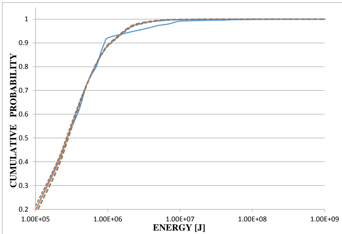
Fig.4. Seismic energy distribution curves from the main syncline region (1987 – 2012). Blue – empirical (ECD), red – theoretical (CDF), greys – 5% confidence intervals for CDF
