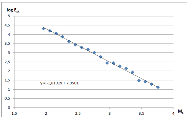
Fig.3. Spatially and temporally averaged coefficient b ~ 1.82 estimated for the whole USCB (from the years 1987 – 2012). E sk – cumulated energy, M L – local magnitude
