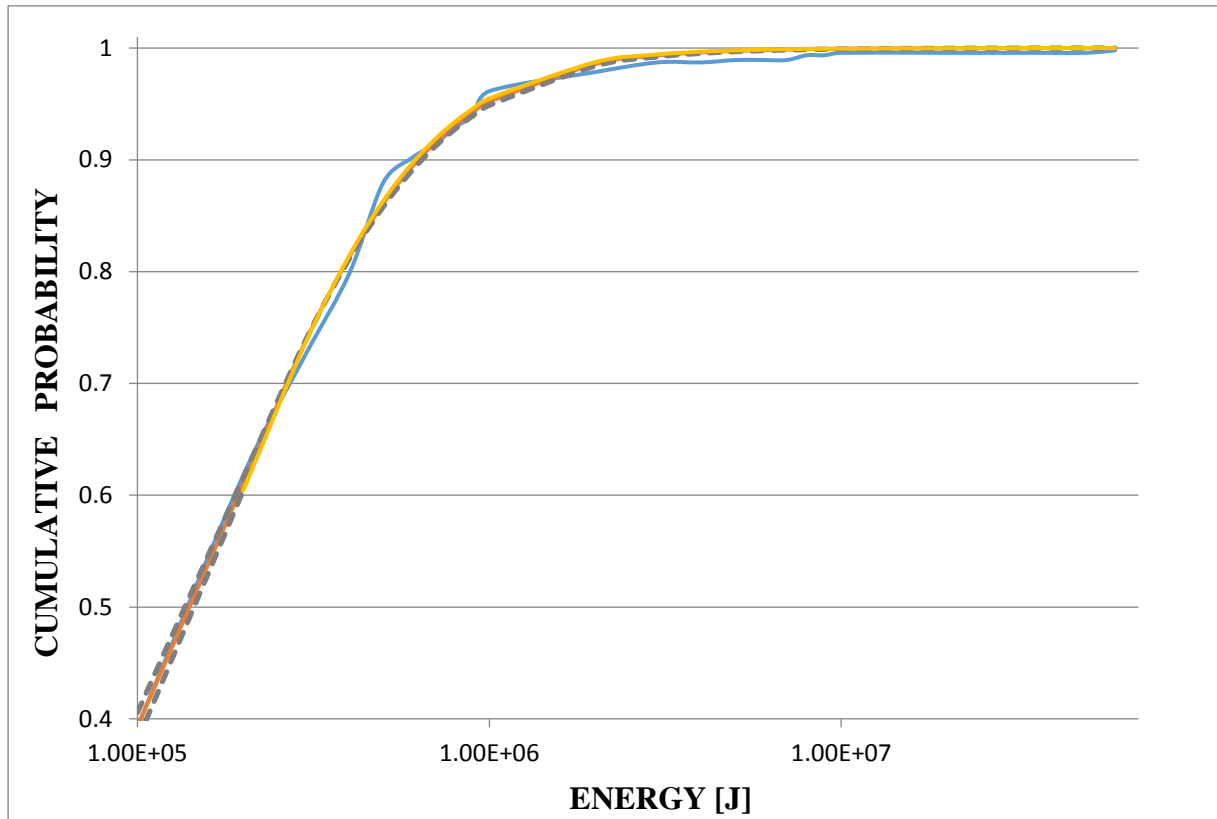
Fig.7. Seismic energy distribution curves from the Kazimierz syncline region (1987 – 2012). Blue – empirical (ECD), red – theoretical (CDF), greys – 5% confidence intervals for CDF
