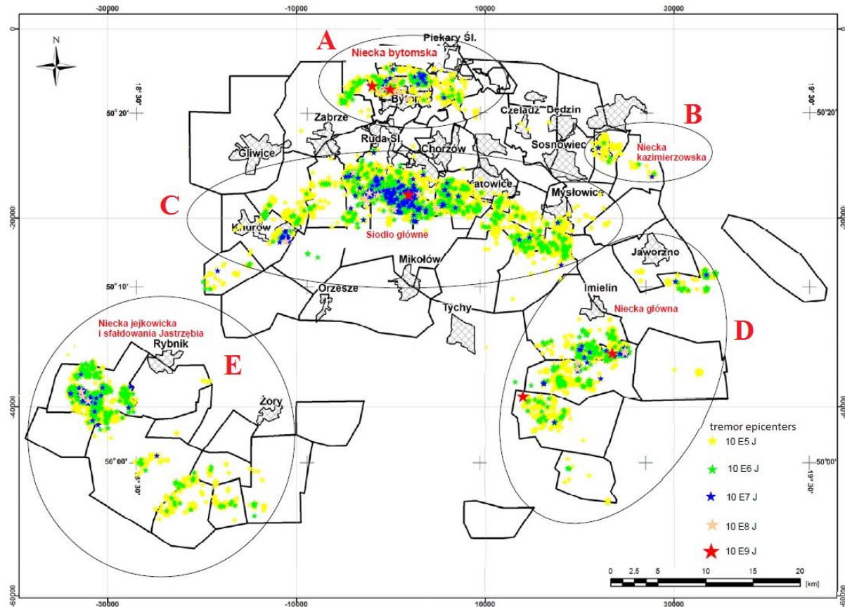
Fig.1. Localizations of strong seismic phenomena (energy E \geq 10^5 J) in the Upper Silesian Coal Basin from the years 1987-2012 on background of mining areas (after Stec, Lurka, 2013, modified) A – the Bytom syncline area, B – the Kazimierz syncline area, C – the main anticline area, D – the main syncline area, E – the Jejkowice syncline and Jastrzębie fold zone (Rybnik Coal District)
