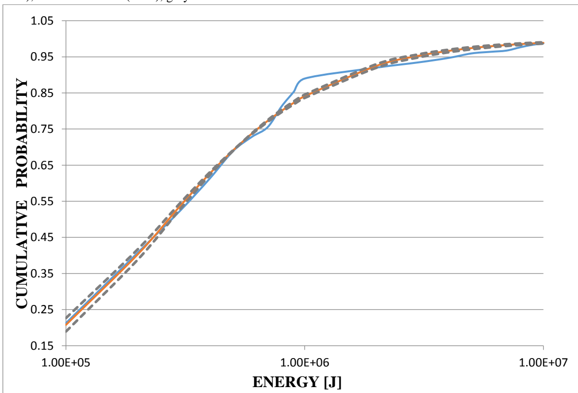
Fig.10. Seismic energy distribution curves for low-energy shocks from the main antycline region (1987 – 2012). Blue – empirical (ECD), red – theoretical (CDF), greys – 5% confidence intervals for CDF
