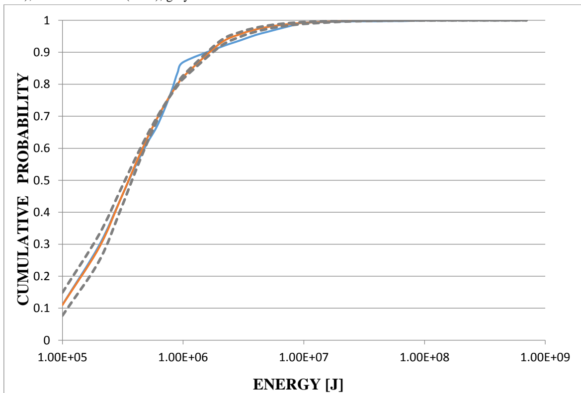
Fig.8. Seismic energy distribution curves from the Jejkowice syncline and Jastrzębie fold zone (Rybnik Coal District) (1987 – 2012). Blue – empirical (ECD), red – theoretical (CDF), greys – 5% confidence intervals for CDF
