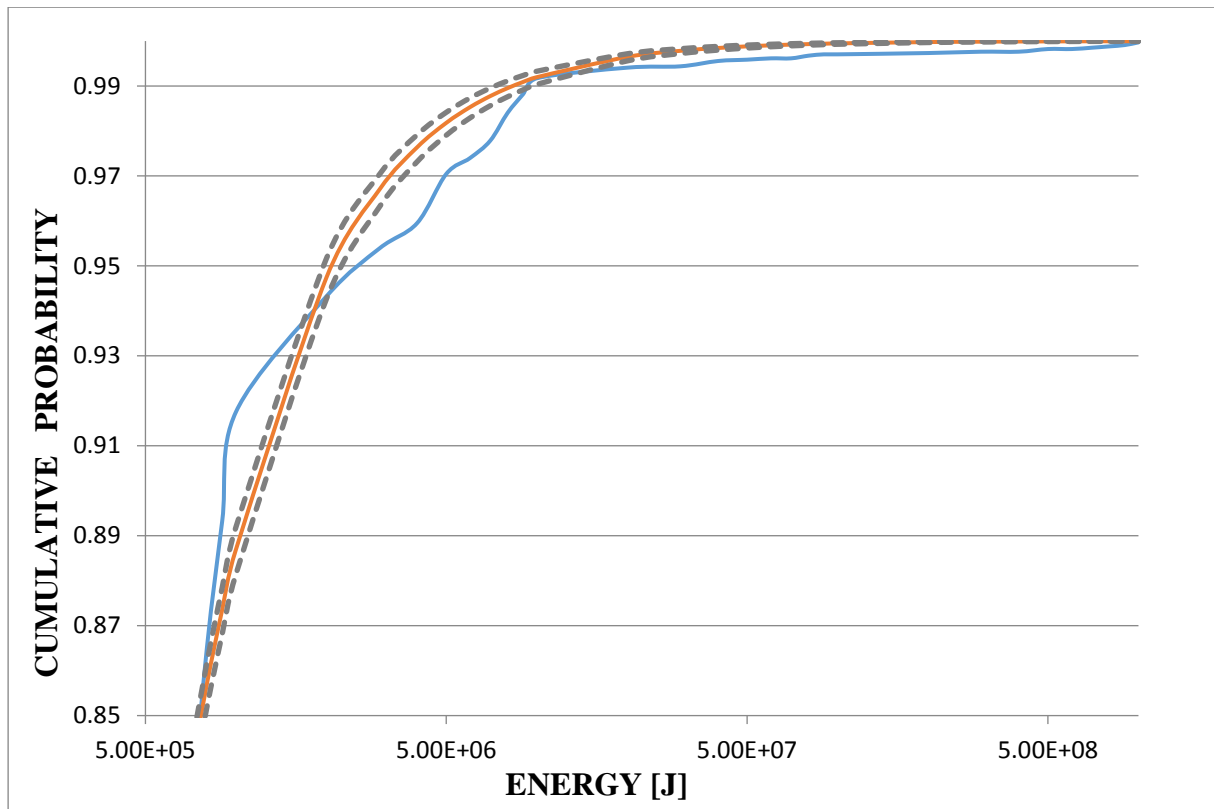
Fig.14. Seismic energy distribution curves for high-energy shocks from the Bytom syncline region (1987 – 2012). Blue – empirical (ECD), red – theoretical (CDF), greys – 5% confidence intervals for CDF
