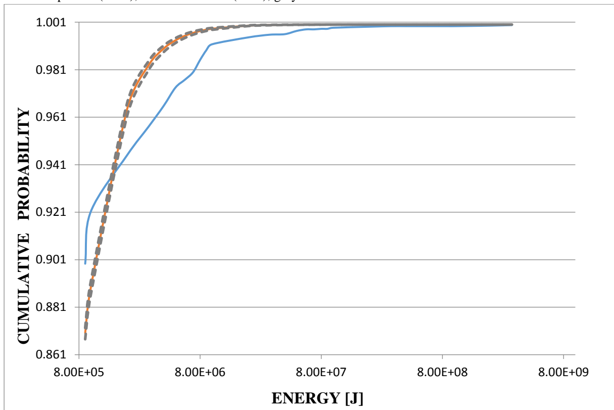
Fig.6. Seismic energy distribution curves for high-energy shocks from the main syncline region (1987 – 2012). Blue – empirical (ECD), red – theoretical (CDF), greys – 5% confidence intervals for CDF
