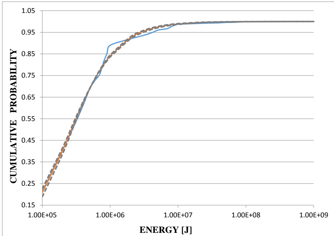
Fig.9. Seismic energy distribution curves from the main antycline region (1987 – 2012). Blue – empirical (ECD), red – theoretical (CDF), greys – 5% confidence intervals for CDF
