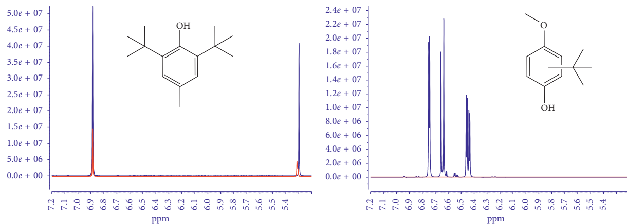
FIGURE 4: Comparison of BHT (a) and BHA (b). The blue ^1\text{H} NMR spectra show the signals of a direct measurement in cyclohexane/acetone- d_6 , while the red spectra represent the result of the SPE cleanup. While BHA is completely removed by SPE, a considerable amount of BHT remains.
