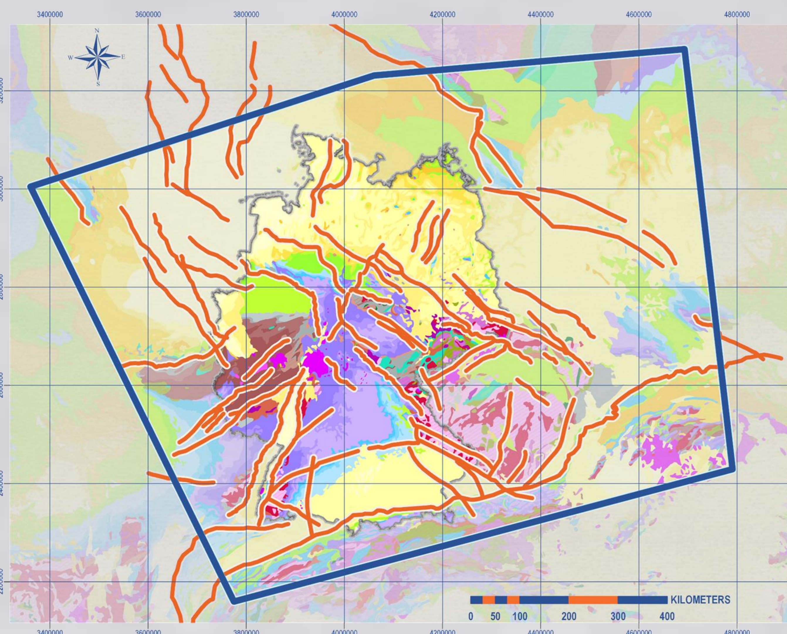
Fig. 3: Model area with major faults on a geological overview map of Europe.
