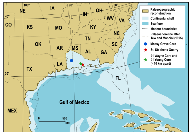
Figure 1. Palaeogeographic reconstruction showing location of the Mossy Grove, #1 Wayne and #1 Young cores, as well as St. Stephens Quarry outcrop. Main North American palaeogeography at \sim 35 \text{ Ma} follows Deep Time Maps™ ( https://deeptimemaps.com/ , last access: 16 October 2018).
