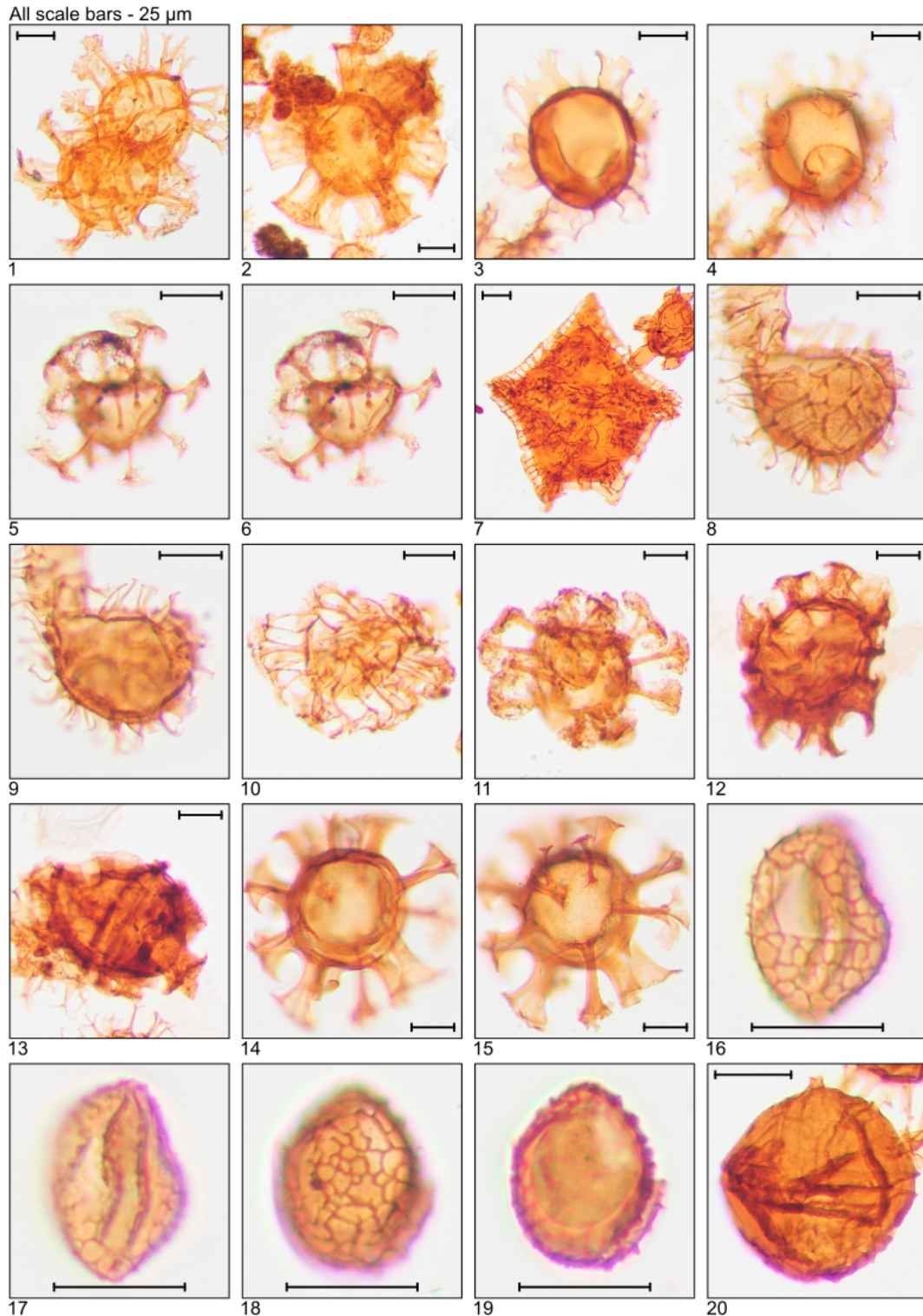
Plate 1. Illustration of taxa and sample or slide number. (1) Achomospaera alcicornu (MG55; 16.8 m; U15). (2) Araneospaera araneosa (MG479; 146.0 m; C19-1). (3, 4) Areoligera sentosa (MG423; 128.9 m; C7). (5, 6) Areospaeridium diktyoplokum (MG243; 74.1 m; C11-1). (7) Charlesdownia coleothrypta (MG271; 82.6 m; L17-1). (8, 9) Cleistosphaeridium ancyreum (MG55; 16.8 m; N23-1). (10) Cleistosphaeridium polypetellum (MG499; 152.1 m; D9). (11) Cordosphaeridium cantharellus (MG215; 65.5 m; C11-1). (12, 13) Cordosphaeridium fibrospinosum (MG383; 116.7 m; D12; MG371; 113.1 m; E18-2). (14, 15) Cordosphaeridium inodes (MG347; 105.8 m; C15). (16–19) Corrudinium incompositum (MG59; 18.0 m; G37, K11-2). (20) Cribroperidinium tenuitabulatum (MG363; 110.6 m; C18-2).
