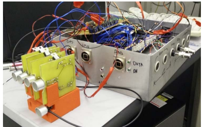
Fig. 6 Optimised MIMO sensor array housing with the sensor modules and the data acquisition box
