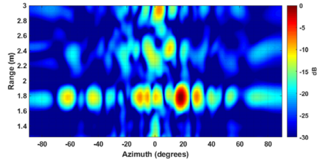
Fig. 13 Target at 20 degrees; range-angle map
