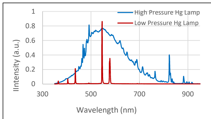
Figure 7. The spectra of a high-pressure mercury lamp and a low-pressure mercury lamp investigated as potential light sources for the redesigned photoelectric effect apparatus (to be used with a monochromator wavelength selector)
