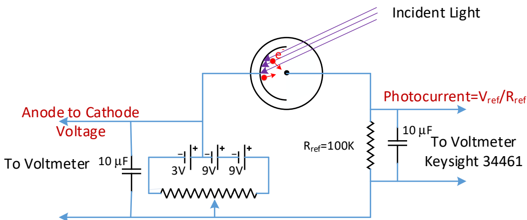
Figure 4. Circuit diagram of the photoelectric effect apparatus
