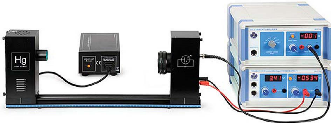
Figure 2. Photoelectric effect commercial experimental apparatus from PASCO [7]
