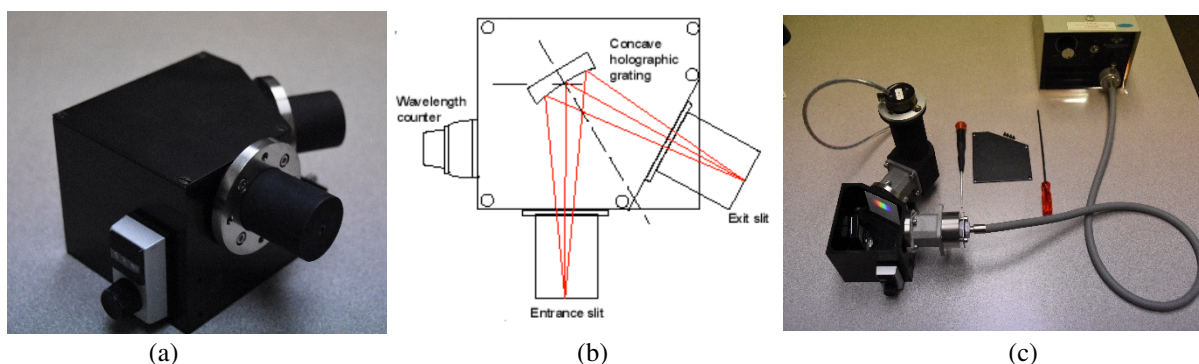
Figure 5. The Horiba H10-61 compact monochromator used in the redesigned photoelectric effect apparatus (a), the light path through the monochromator (b), and the monochromator outfitted with the phototube mounted on the exit slit (c)
