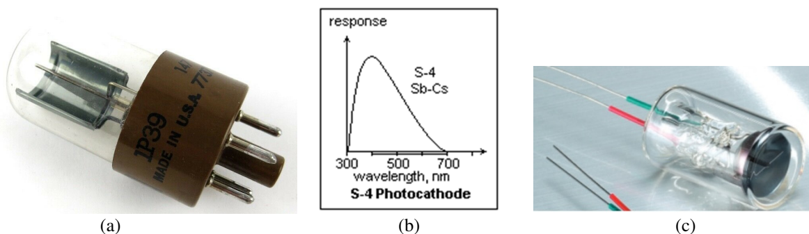
Figure 6. The side-window RCA/GE/Cetron 1P39 (929) vacuum phototube (a), its so-called S4 spectral response curve (b), and the front-end-window R-414 Hamamatsu phototube (c)
