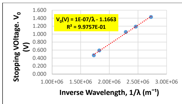
Figure 8. Stopping voltage as a function of inverse wavelength for the 1P39 photoelectric tube. The resulting value for Planck's constant is 5.34 \times 10^{-34} \text{ J} \cdot \text{s} , which is 18% off from accepted value. The work function of the cathode is 1.166 eV
