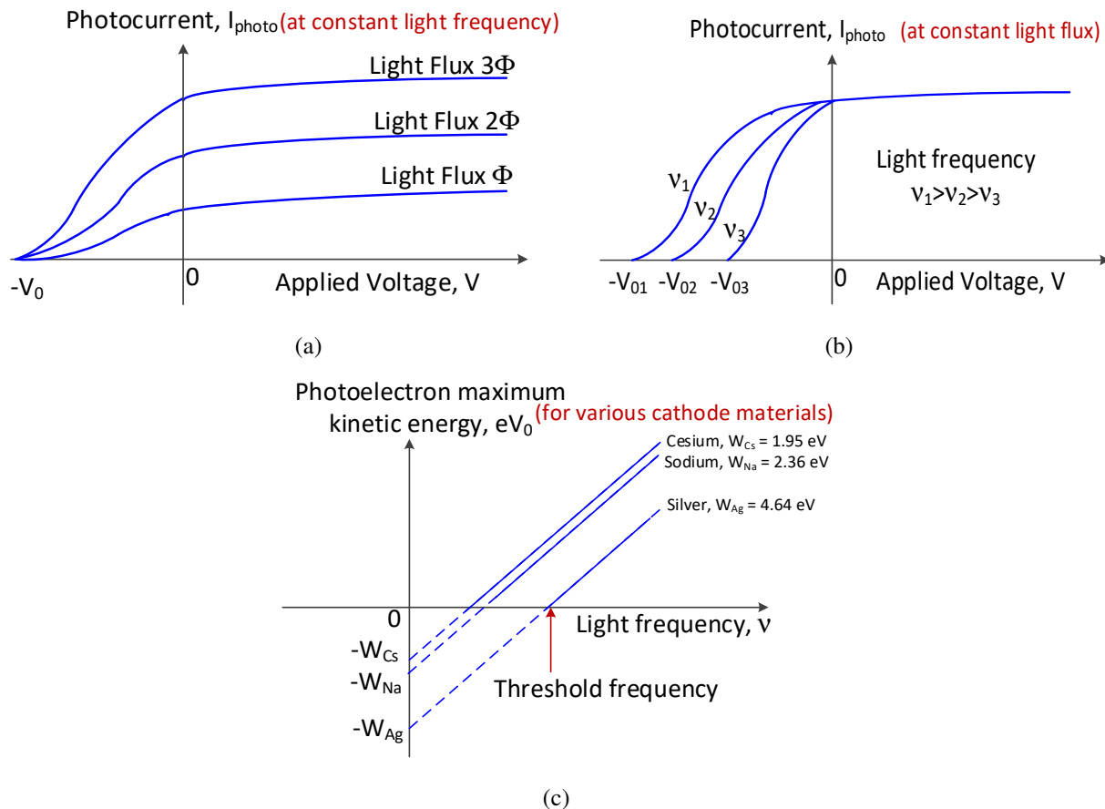
Figure 1. A graphical summary of the properties of the photoelectric effect, as predicted by Einstein's 1905 equation for the effect (Eqn. 4) and verified experimentally (in a qualitative way) by Lenard between 1900 and 1902
