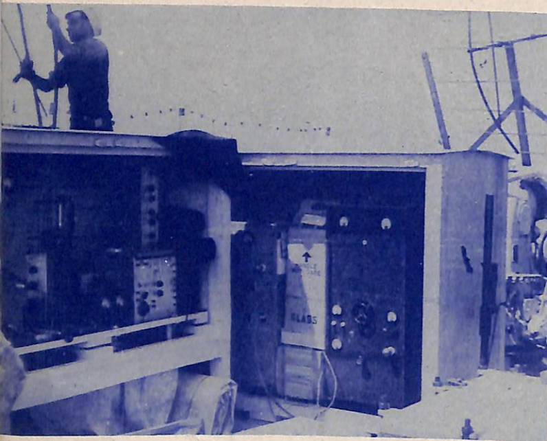
First radar installation on a ship, mounted on a gun on the old USS LEAHY in 1937.
