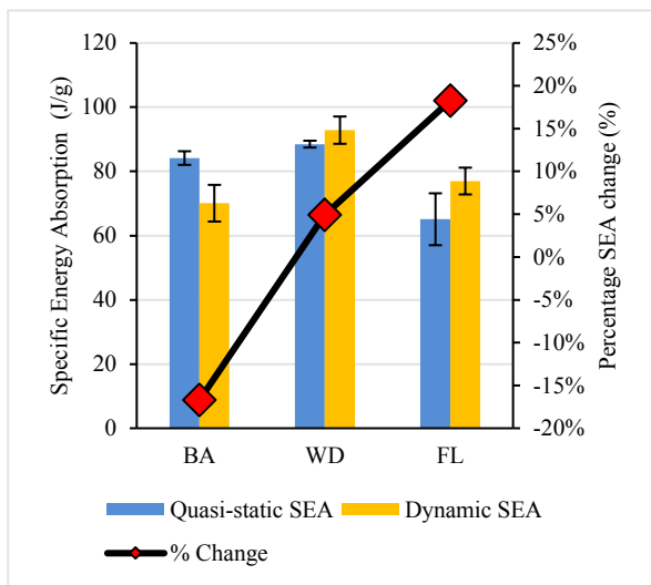
Figure 6: SEA characteristics of crushed specimens.
