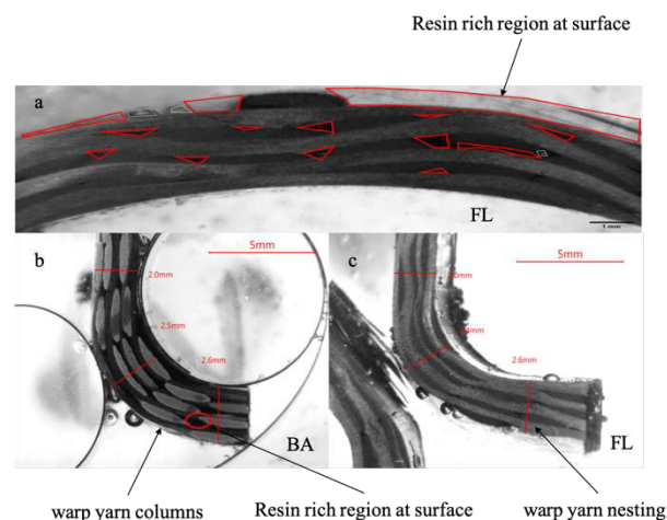
Figure 3 : Micrographs of bend radii in omega-shaped specimens: (a) semi-circle in FL; (b) flange in BA; and (c) flange in FL
