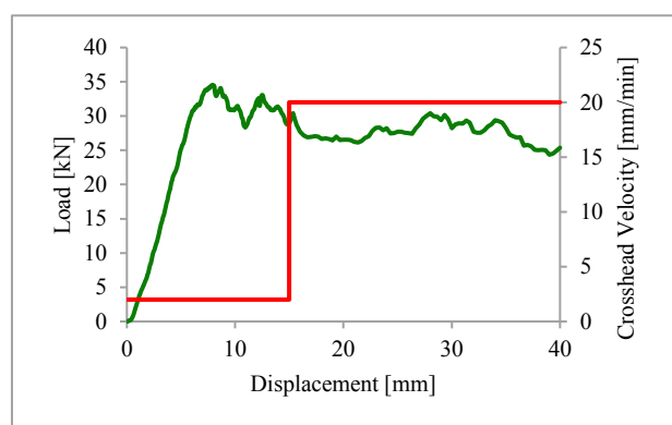
Figure 4: Typical load displacement curve showing quasi-static crush in a WD specimen.
