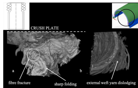
Figure 7: Micro-CT images showing a cross-section view of (a) progressive folding and (b) external yarn slippage in FL specimens.
