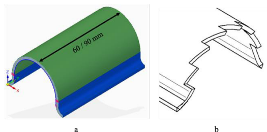
Figure 2: (a) Omega-shaped specimen (b) saw-tooth trigger
