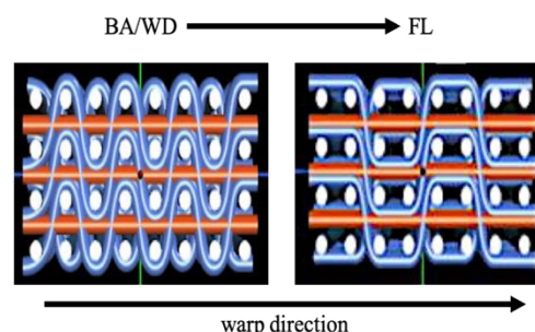
Figure 1: Comparison between weave architectures in BA/WD specimens and FL specimens.
