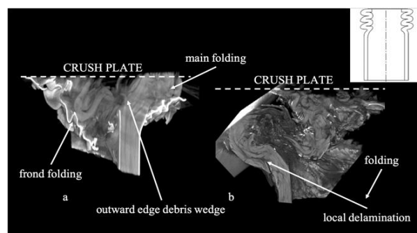
Figure 5: Micro-CT images showing cross-section view of progressive folding events in (a) BA and (b) WD specimens.
