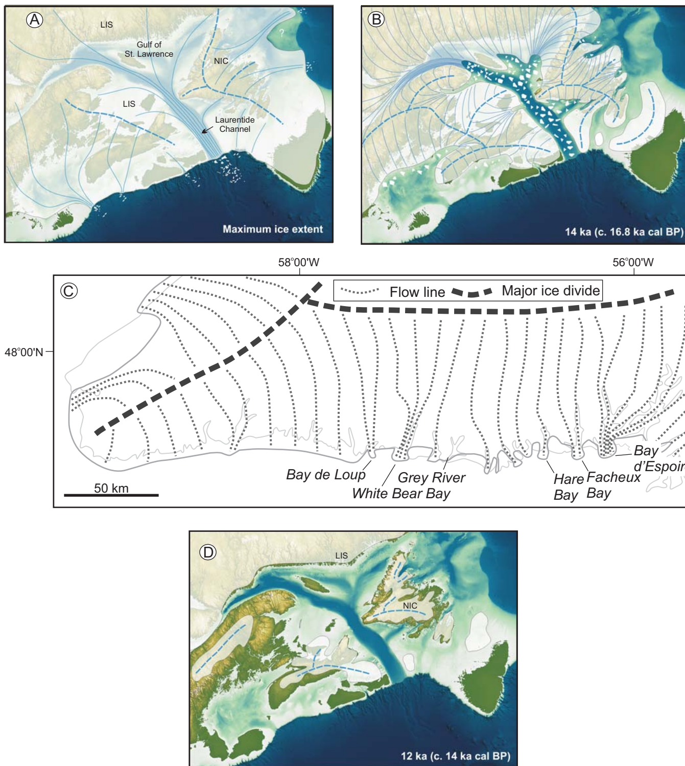
Figure 2. A) Maximum ice extent during the Late Wisconsinan glaciation. Dashed blue lines are major ice divides and solid blue lines generalized flow lines. The Laurentide Ice Sheet (LIS) extended over mainland Canada and coalesced with the Newfoundland Ice Cap (NIC) over the Island of Newfoundland; B) Calving is believed to be responsible for a rapidly changing ice margin at 14 ka BP, resulting in ice being removed from the Gulf of St. Lawrence, and isolation of the Newfoundland Ice Cap; C) Ice margin 13.5 ka BP along the south coast of Newfoundland showing lobate ice margins in Bay de Loup, White Bear Bay, Hare Bay, Facheux Bay and Bay d'Espoir; D) Ice margins and major ice divides (dashed blue lines) at 12 ka BP. Illustrations A, B and D are adapted from Shaw et al. (2006); illustration C is adapted from Shaw (2003).
