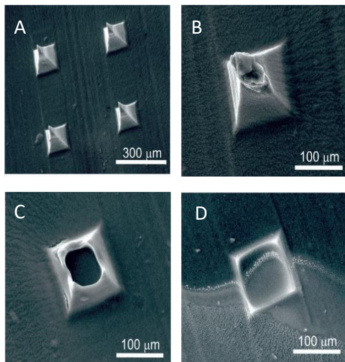
Figure 2. Scanning electron micrographs of the cellulose acetate phthalate microneedles upon exposure to pH 8 Britton Robinson buffer. Recorded at (A) 0, (B) 1, (C) 3, and (D) 5 minutes.
