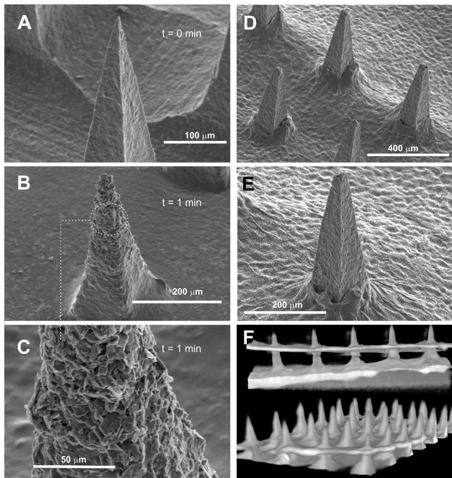
Figure 3. Scanning electron micrographs of the C-CAP microneedles before (A) and after (B) 1 minute exposure to pH 8 Britton Robinson buffer. Dissolution of the CAP polymer leaving carbon platelets is highlighted in (C). Scanning electron micrographs (D,E) and computerized tomography (F) of microneedles piercing of needles through de-fleshed tomato skin.
