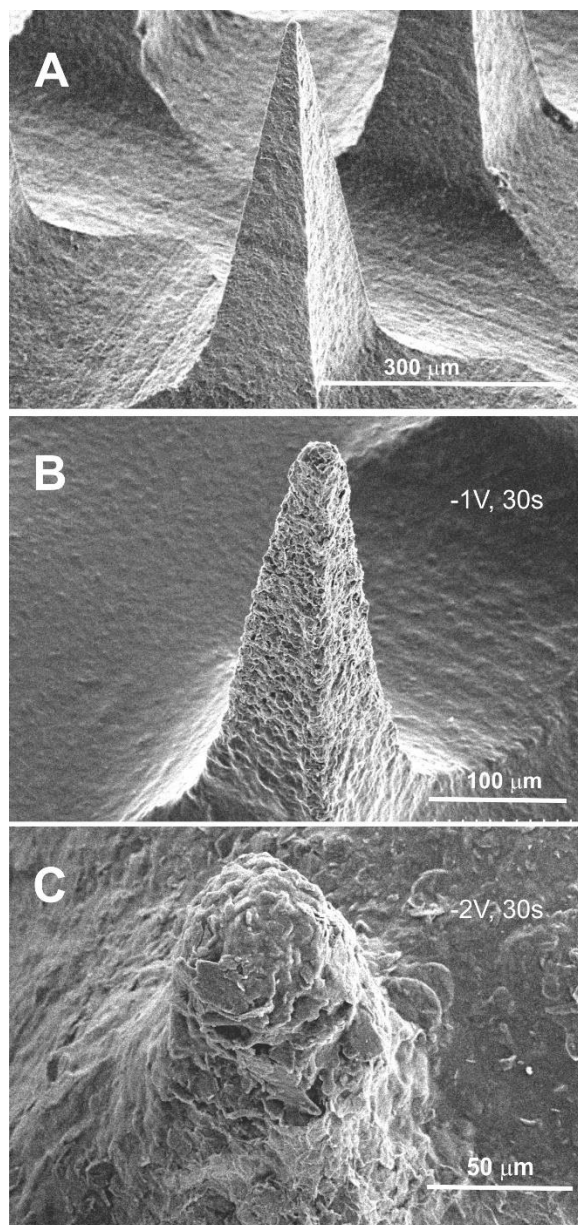
Figure 8. Scanning electron micrographs of the C-CAP-Pd microneedles after poisoning the electrode at a reducing potential. A) Open circuit. B) -1 V for 30 s. C) -2 V for 30 s.
