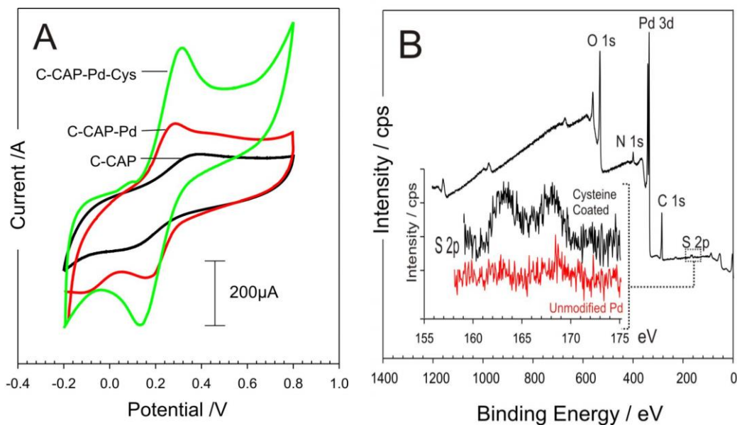
Figure 5. A) Cyclic voltammograms comparing the response of the C-CAP and C-CAP-Pd microneedles to 2 mM Ferrocyanide before and after modification with palladium and cysteine. Scan rate: 50 mV/s. B.) XPS spectra highlighting the modification of C-CAP-Pd microneedles with cysteine.
