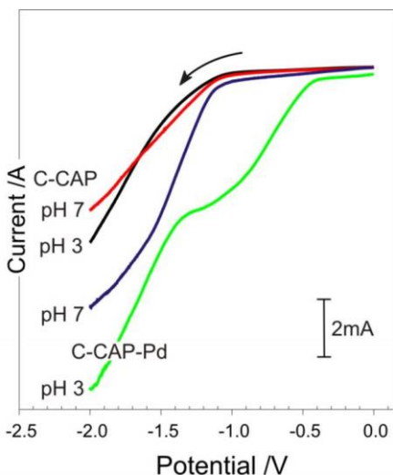
Figure 6. Linear sweep voltammograms of the unmodified and Pd coated microneedles in pH 3 and pH 7 Britton Robinson buffer. Scan rate: 50 mV/s.
