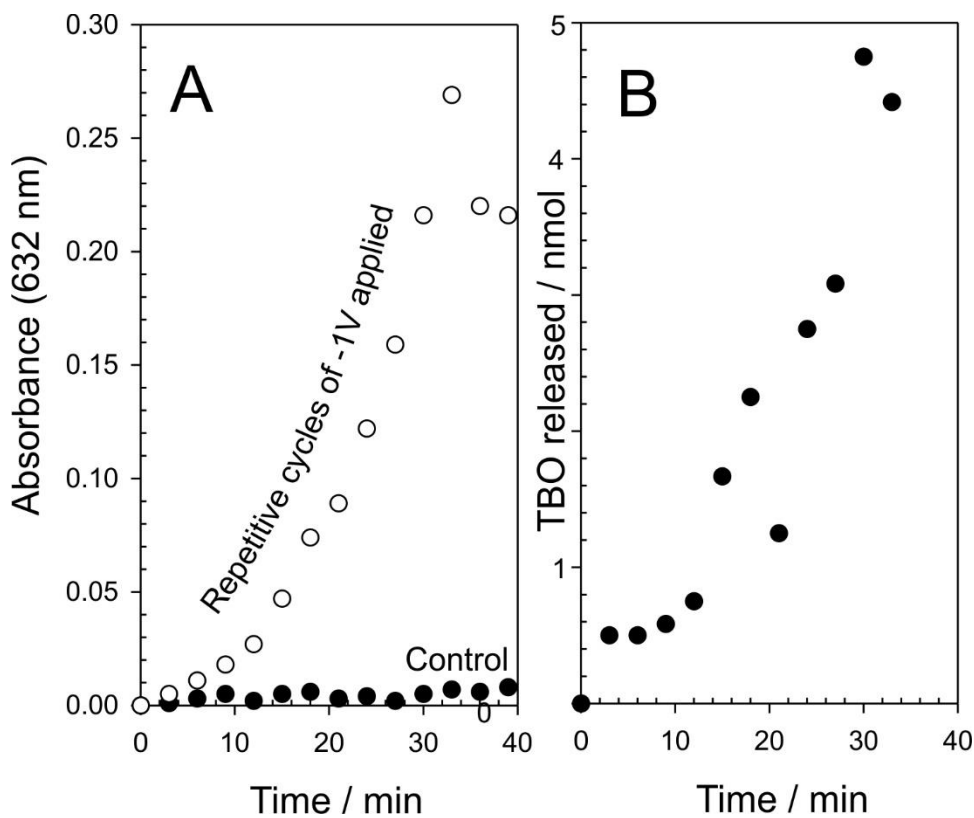
Figure 10. The effect of repetitive applying a potential (-1V, 300s) on the release of Toluidine Blue into pH 5 buffer (A) and the corresponding yield per cycle (B)
