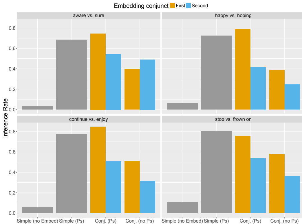
Figure 6 Mean inference rates of p per condition by Trigger and No-Ps control in Experiment 2
