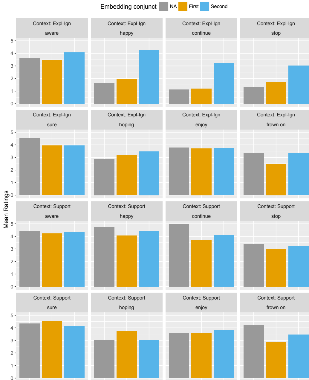
Figure 8 Mean acceptability ratings per Context and Order by Trigger in Experiment 3
