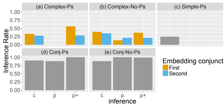
Figure 5 Mean inference rates for fillers by inference type and conjunct order (where applicable) in Experiment 1
