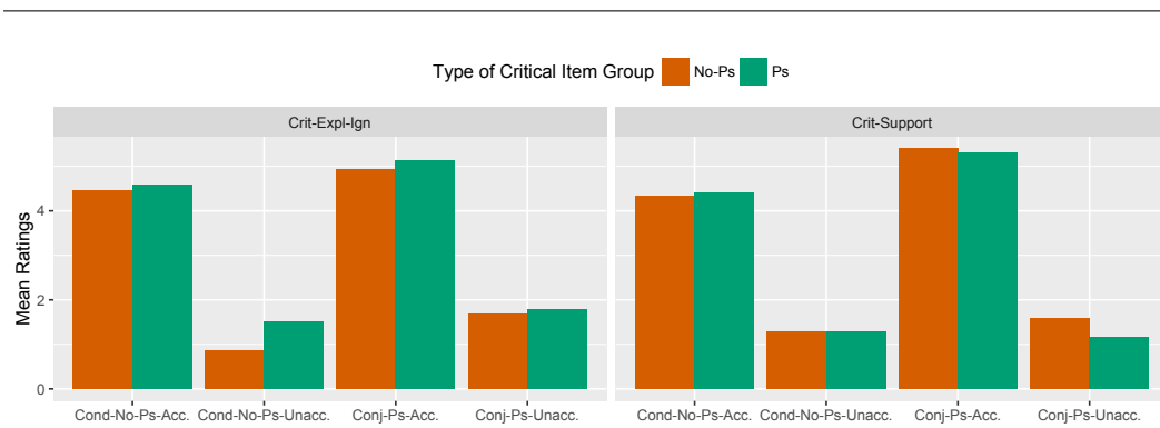
Figure 9 Mean acceptability ratings for fillers by type and between-subject factor groups (Context and Embedding Type for critical items)
