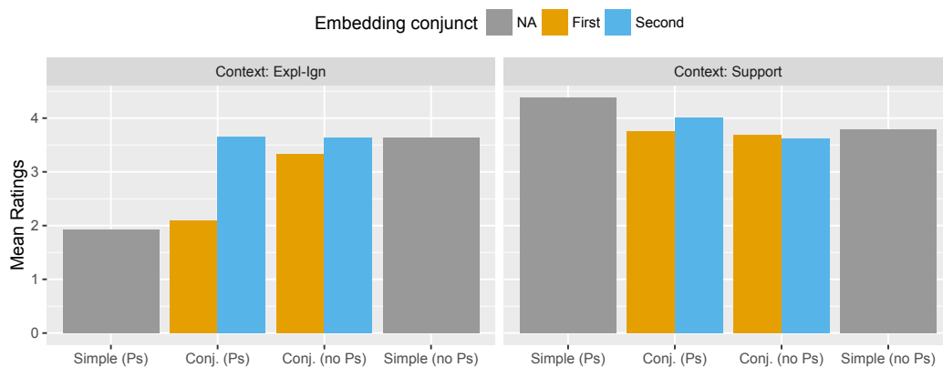
Figure 3 Mean acceptability ratings by context and condition in Experiment 3
