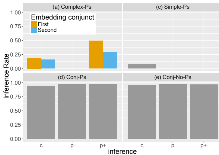
Figure 7 Mean inference rates for fillers by inference type and conjunct order (where applicable)
