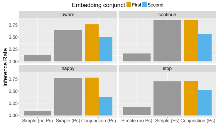
Figure 4 Mean inference rates of p per condition by Trigger in Experiment 1
