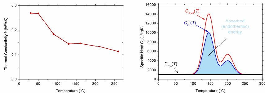
Figure 3. Temperature dependent thermo-physical properties of gypsum plasterboard.
