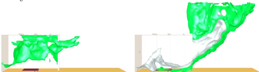
Figure 5. Predictions of C_{18}H_{38} vapour volume fraction iso-surfaces (white: 0.001, green: 0.01), 35 s (left) and 300 s (right) after fire initiation.
