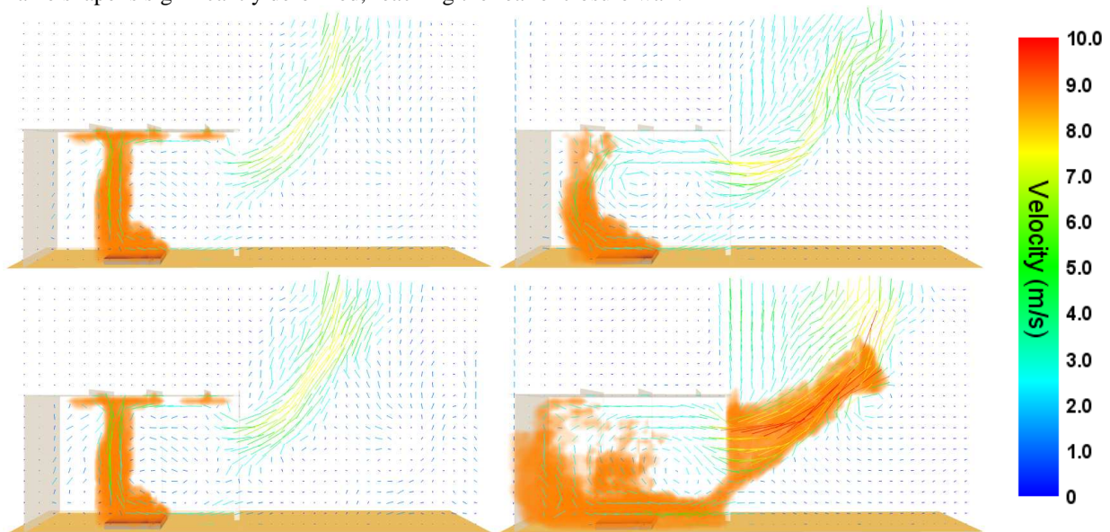
Figure 4. Predictions of gas mixture velocity and flame location, for test cases GP (top) and GP+PCM (bottom), 8 s (left) and 300 s (right) after fire initiation.
