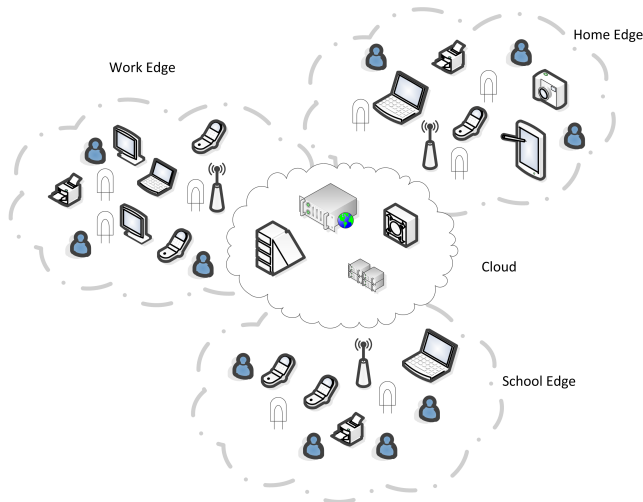
FIGURE 1. Cloud and edge computing.
