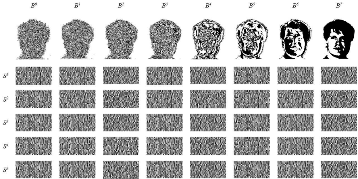
FIGURE 4. Secret shares for all bit planes B^0, B^1, B^2, B^3, B^4, B^5, B^6, and B^7 .
