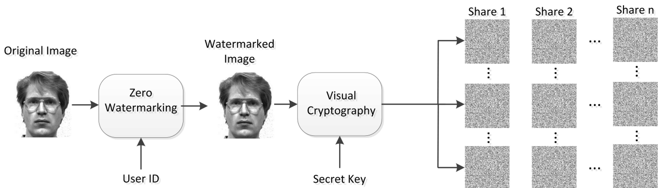
FIGURE 2. The zero-watermarking and visual cryptography procedures at the edge.
