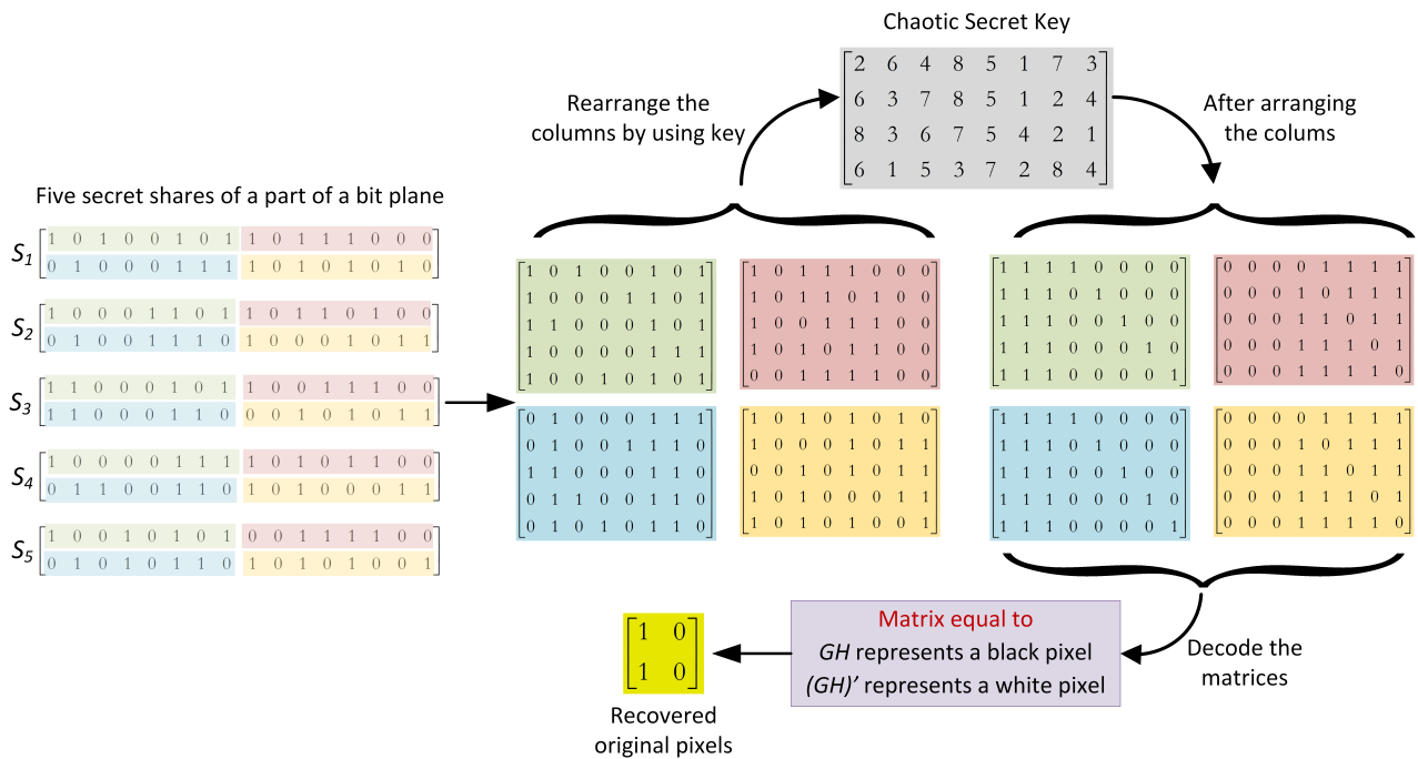
FIGURE 5. The decryption process.
