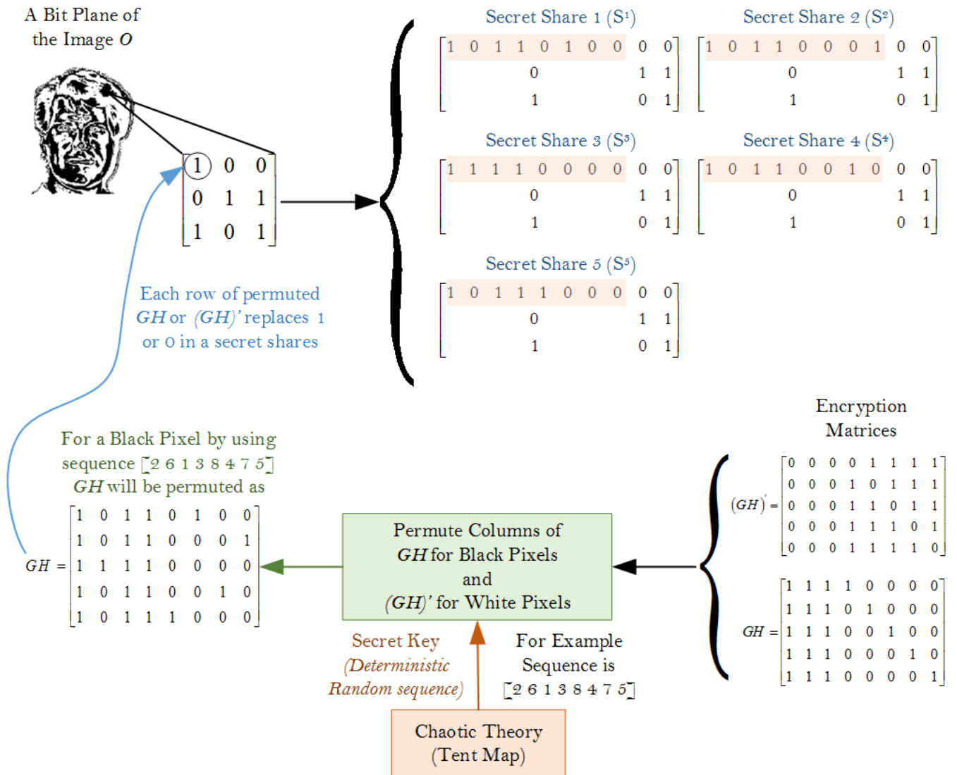
FIGURE 3. The encryption process.
