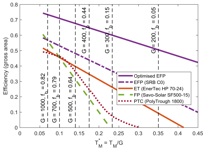
Figure 16. Simulated normal-incidence efficiency of an optimised evacuated flat plate compared with commercial EFP, evacuated tubes, flat plate and trough collectors operating at T_M = 70^\circ\text{C} .
