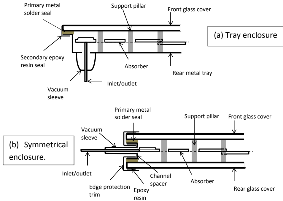
Figure 6. Cross-sections showing the coolant feed pipe connections, edge seals and pillar geometry: (a) tray enclosure, (b) symmetrical enclosure.
