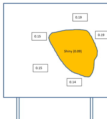
Figure 4. (a) Emissivity (%) for top surface of the symmetrical absorber, (b) Approximate emissivity of lower surface; the plating of this absorber resulted in very little black chrome on the rear face.
