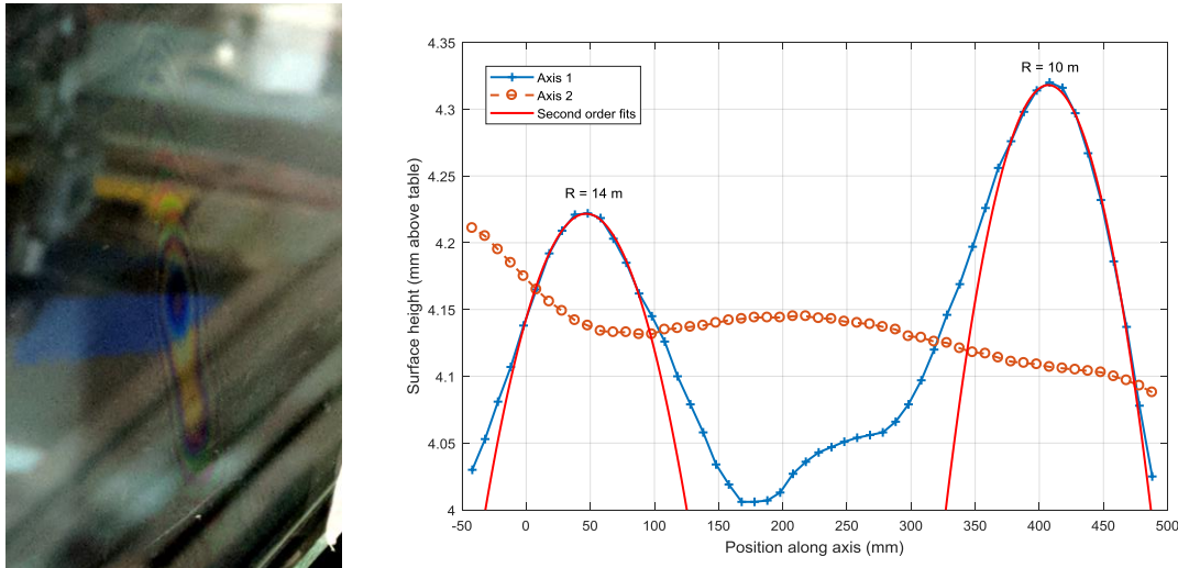
Figure 8. (a) “Newton’s ring” interference fringes showing a contact point between 4 mm toughened and plain glass, (b) Surface profile of this toughened glass sheet.
