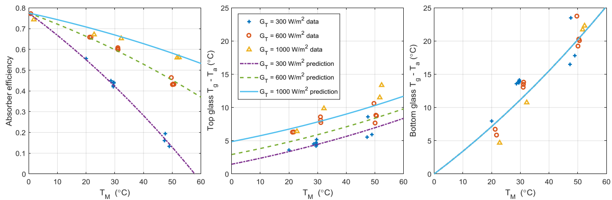
Figure 15. Comparison of symmetrical enclosure data with simulations (evacuated, fan on); input parameters as Table 1.
