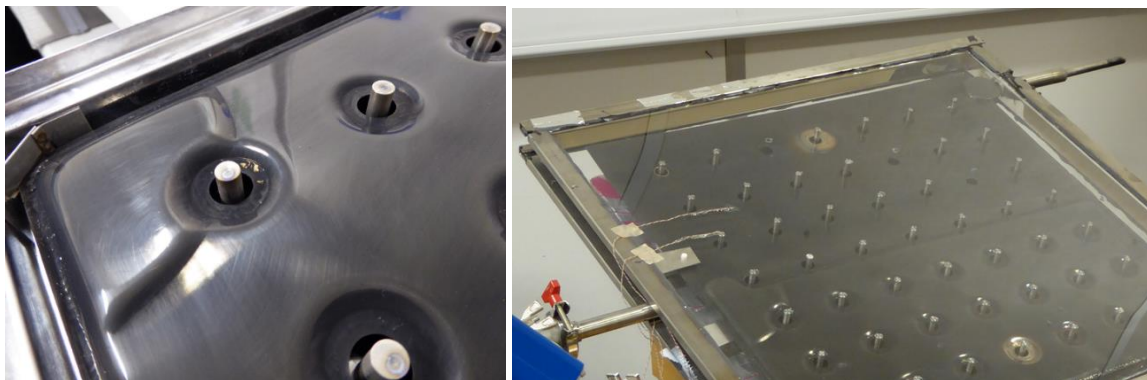
Figure 7 . (a) “tray” enclosure details showing corner location and deeper absorber section above the feed pipe. (b) The symmetrical collector being instrumented prior to testing.
