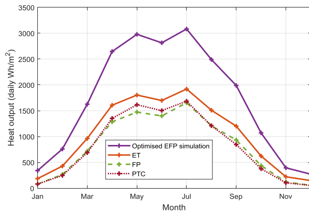
Figure 17. Predicted heat transfer to an 85°C district heating main based on weather station irradiance and ambient temperature for 2011-17.
