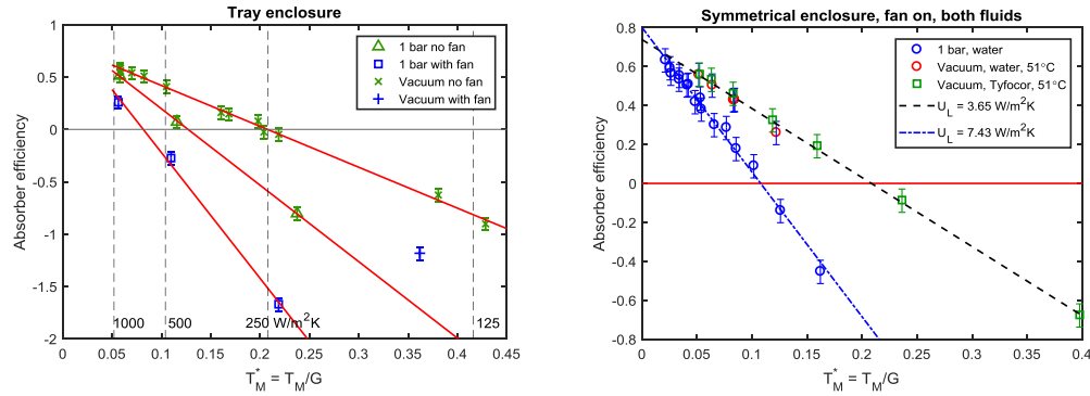
Figure 12. Test results. (a) Efficiencies for the “tray” enclosure, (b) efficiencies for the symmetrical enclosure.
