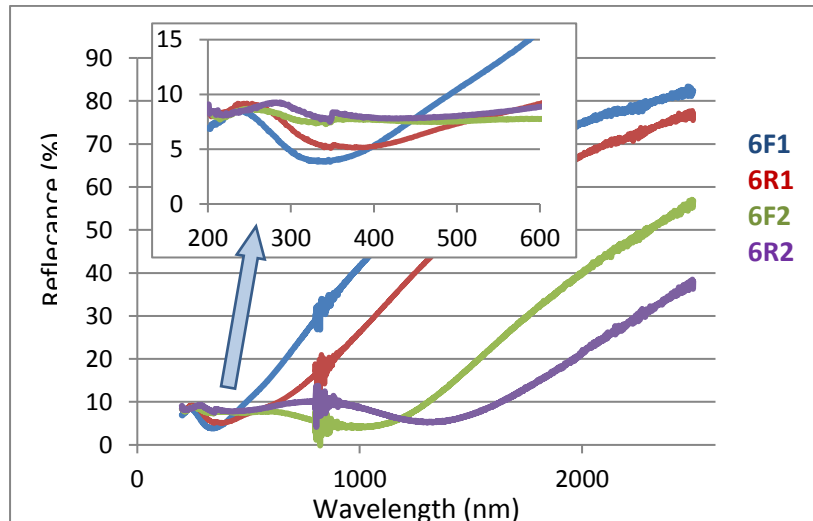
Figure 5. Reflectivity (%) of four plating samples.
