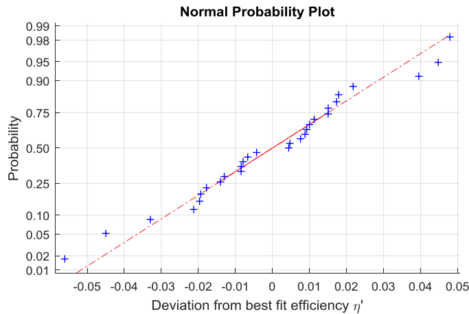
Figure 13. Distribution of deviations from linear regression lines.
