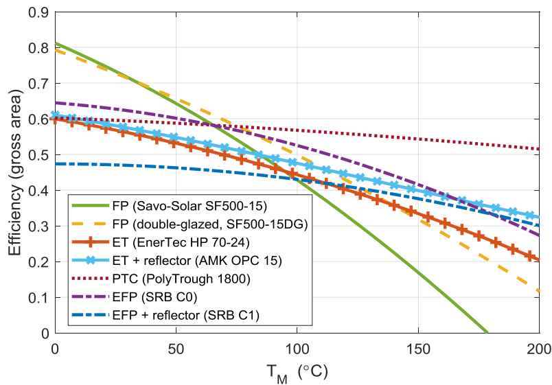
Figure 1. Comparison of published data for solar collector architectures at G_b = 1000 \text{ W/m}^2 . (SPF catalogue [4]; SRB curves from Pauletta [5]).
