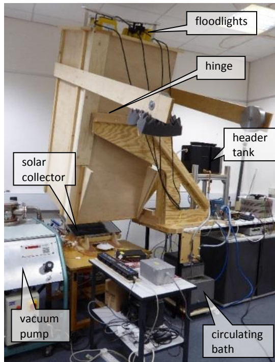
Figure 9. Simulator and instrumentation during “tray” enclosure testing.
