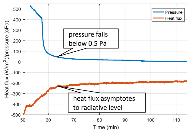
Figure 11. Reduction in heat losses when the internal pressure was suddenly reduced (tray collector).
