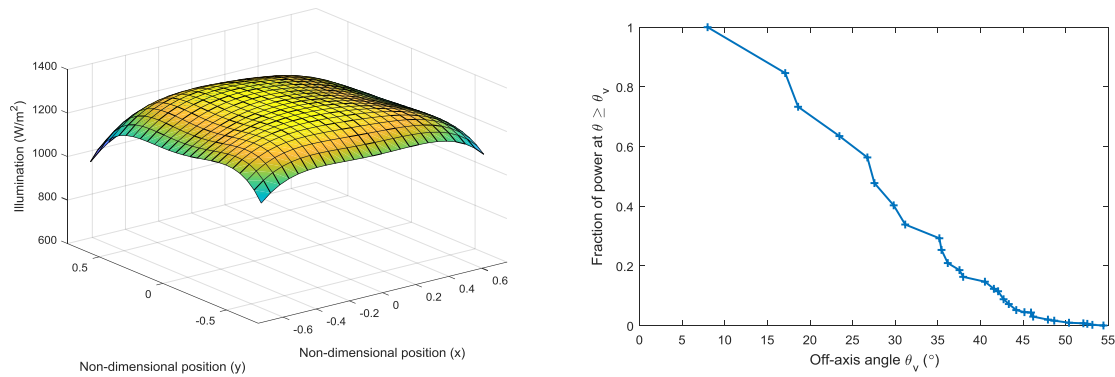
Figure 10. (a) Polynomial surface fit of pyranometer illumination measurements over a 5×5 grid (using all 4 lamps), (b) Predicted cumulative irradiance distribution at the centre of the collector. There is no peak at 0° because the four lamps are arranged symmetrically around the simulator axis; none of them are on-axis.
