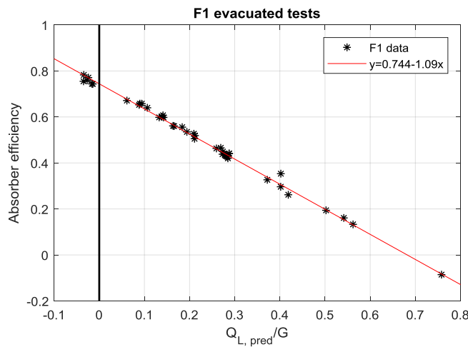
Figure 14. Comparison of experimental heat loss measurements with an emissivity-based model.
