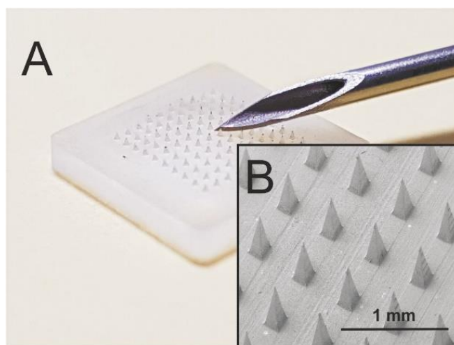
Figure 3. A) Comparison of a microneedle patch (200x200x350 \mu\text{m} ) with a standard hollow-bore needle. B) Electron micrograph of the polystyrene microneedle patch.
