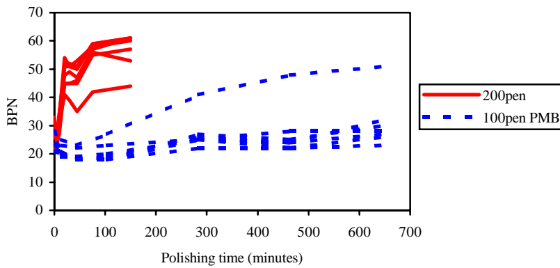
Figure 3 Comparison of change in BPN for a 200pen and 100pen polymer modified binder
