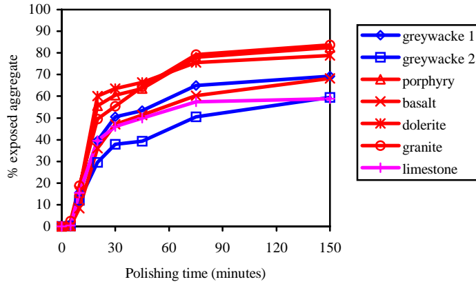
Figure 2 Exposure of aggregate during testing depending on rock type (200pen)
