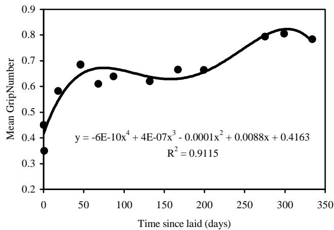
Figure 4 Change in GripNumber with time for a section of 14mm SMA
