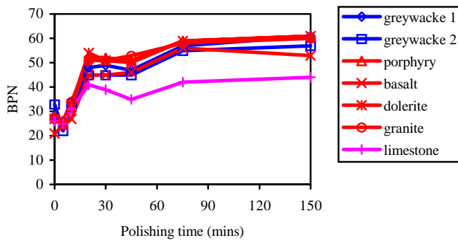
Figure 1 Change in skid resistance during testing depending on rock type (200pen bitumen)
