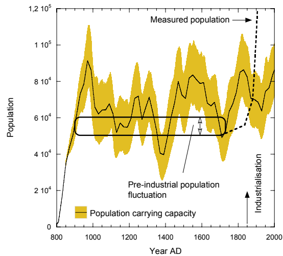
Figure 3: The simulated pre-industrial human population in Iceland
