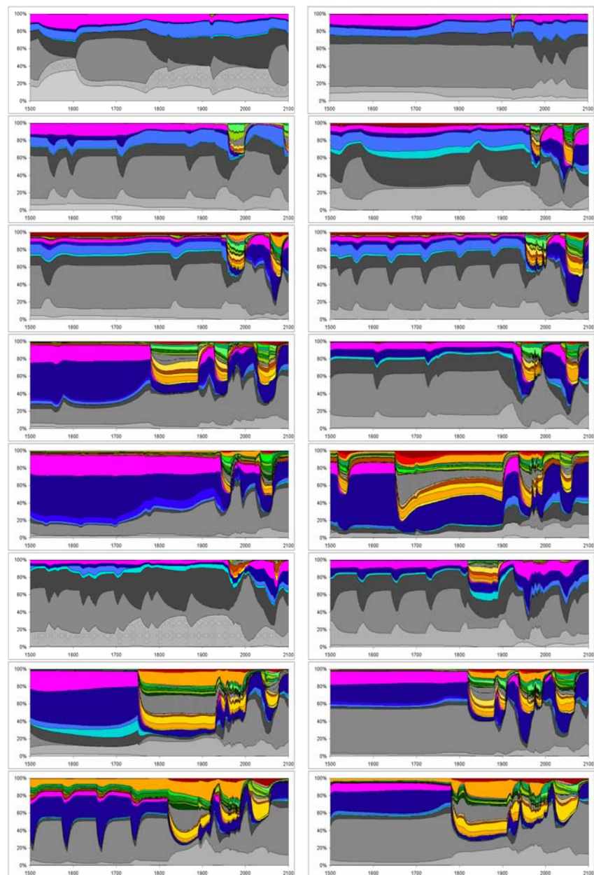
Figure 6. Summary of simulated ground vegetation composition, north (top) to south (bottom) From top right: Högbränna, Brattfors, Storulvsjön, Blåbärskullen, Örlingen, Högskogen, Hensbacka, Höka, Edeby, Söstared, Gyngje, Fagerhult, Timrilt, Bullsäng, Vang, Torup. Gray: lichens and mosses; Blue: heather and ling; Yellow: Grasses; Red: Brackens and ferns; Green: herbaceous plants; Brown: Bushes, bush-like ling and thickets.
