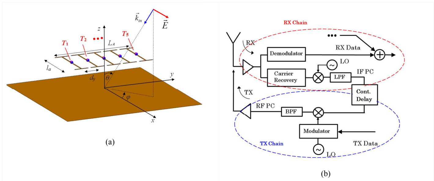
Fig.1. (a) A simulation model of an ultra-compact retrodirective antenna array illuminated by a linearly x -polarized monochromatic PW. The antenna array characteristic size L_a \sim Nd_y \sim 0.5\lambda , N is a number of antenna elements, the inter-element spacings d_y are of order of 0.1\lambda . T_m , n=1,2,\dots,N are the PC antenna ports. The antennas are end-loaded to ensure electric
