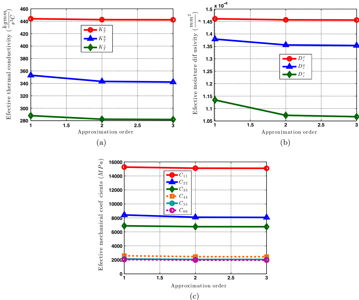
Fig. 10. Diagonal elements of the homogenised matrices \bar{K}_T , \bar{D}_c and \bar{C} in the case of heat transfer, moisture transport and mechanical RVEs.
