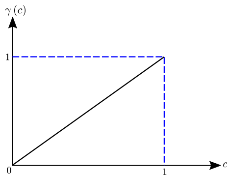
Fig. 6. \gamma(c) versus moisture concentration c .
