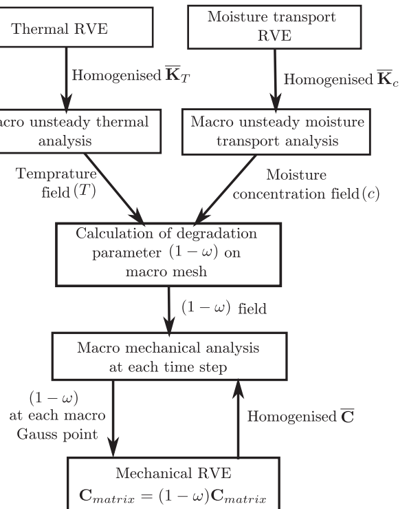
Fig. 7. Flow chart for the computational framework.
