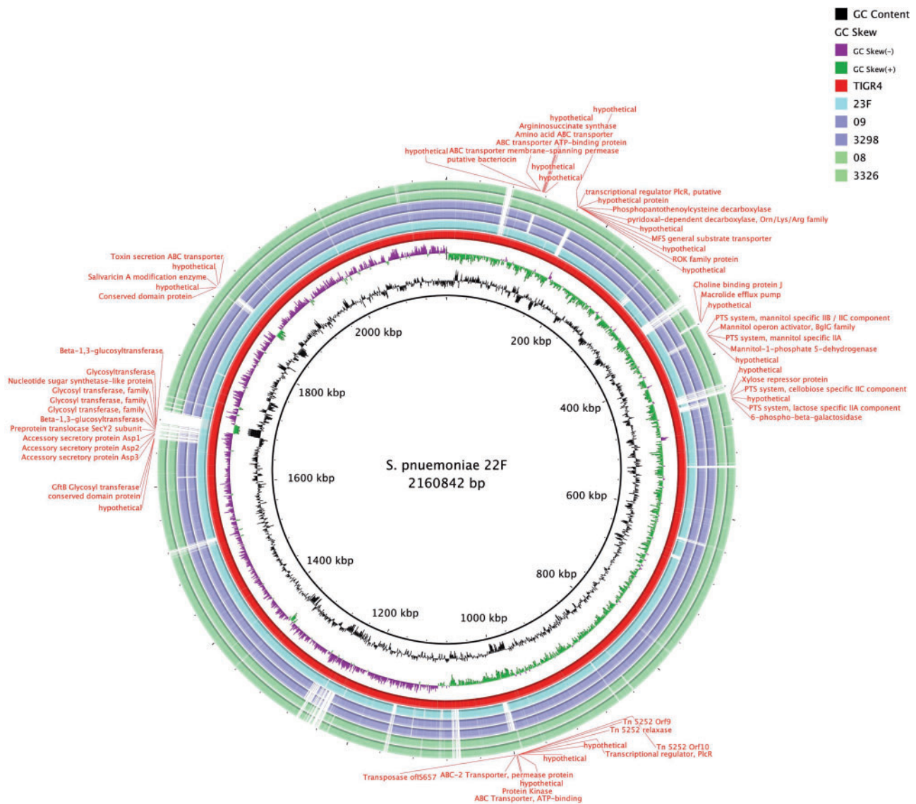
Fig. 3. —Genome comparisons of four Streptococcus pneumoniae serotype 22F isolates against TIGR4 and ATCC 70669 23F. Rings representing ST433 isolates (08 and 3326) are colored green with ST698 isolates (09 and 3298) colored purple. The red labels show regions of gene absences, and gene classifications were derived from TIGR4 annotations in RAST.
