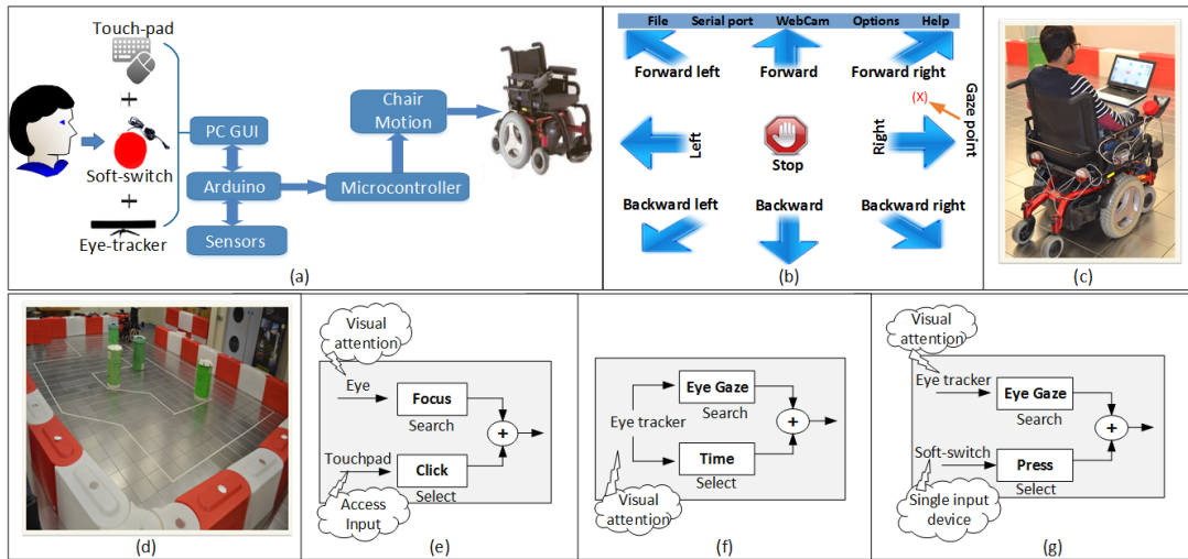
Fig. 1. System overview. (a) Block diagram of the proposed system, (b) Personal computer graphical user interface (PC GUI), (c) Organization of the system components, (d) View of the test trajectory, and (e-g) Proposed models of multimodal interface based on various input modalities, wherein the search and selection of the items are performed by (e) eyes without eye-tracker and laptop touchpad, (f) eye-tracker with dwell time, and (g) eye-tracker with soft-switch.
