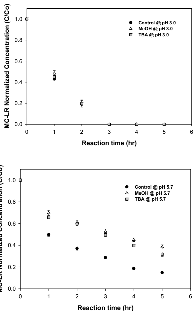
Fig. 1. Photocatalytic degradation of MC-LR with NF-TiO 2 in the absence and presence of methanol and tert -butyl alcohol as •OH scavengers under visible light at a) pH 3.0 b) pH 5.7.
