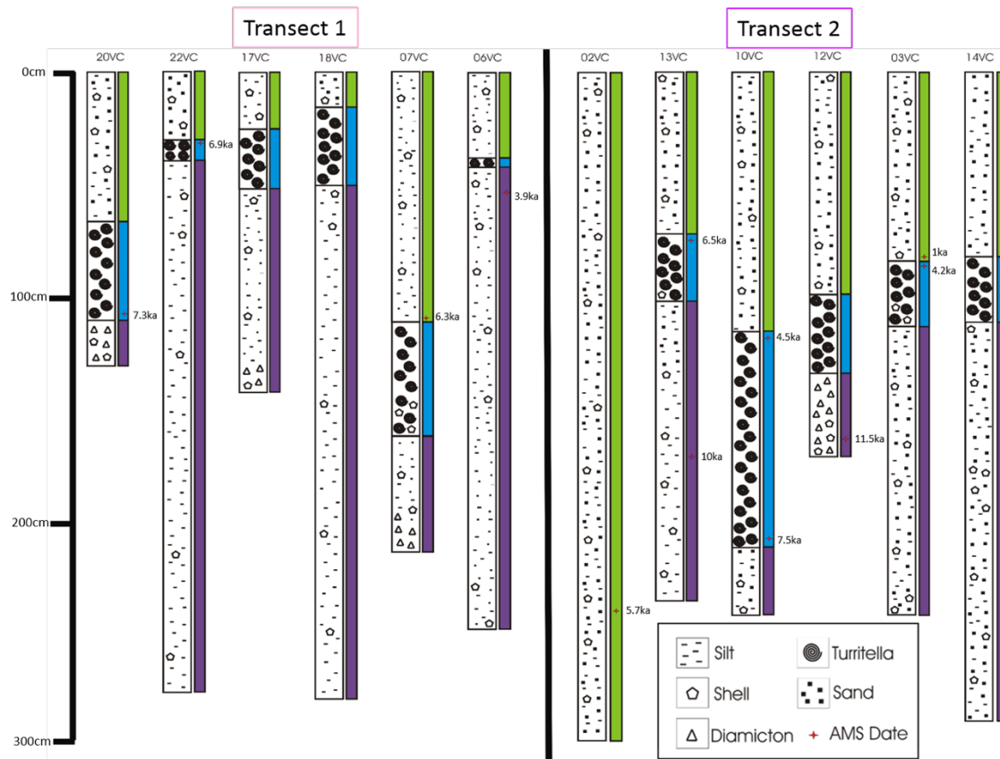
Fig. 2 - Core logs for the longest and more meaningful cores in two transects corresponding approximately to the North and South sounds (Fig. 1). The top lithofacies (green) is a sandy silt and clay facies, which is often followed by a distinct shell hash interlayer (blue) which we named the “ Turritella Layer”. This layer is then underlaid by a fine silty sand facies (purple), with a general lower abundance of microfossils and the occurrence of rare gravel and pebble grains.
