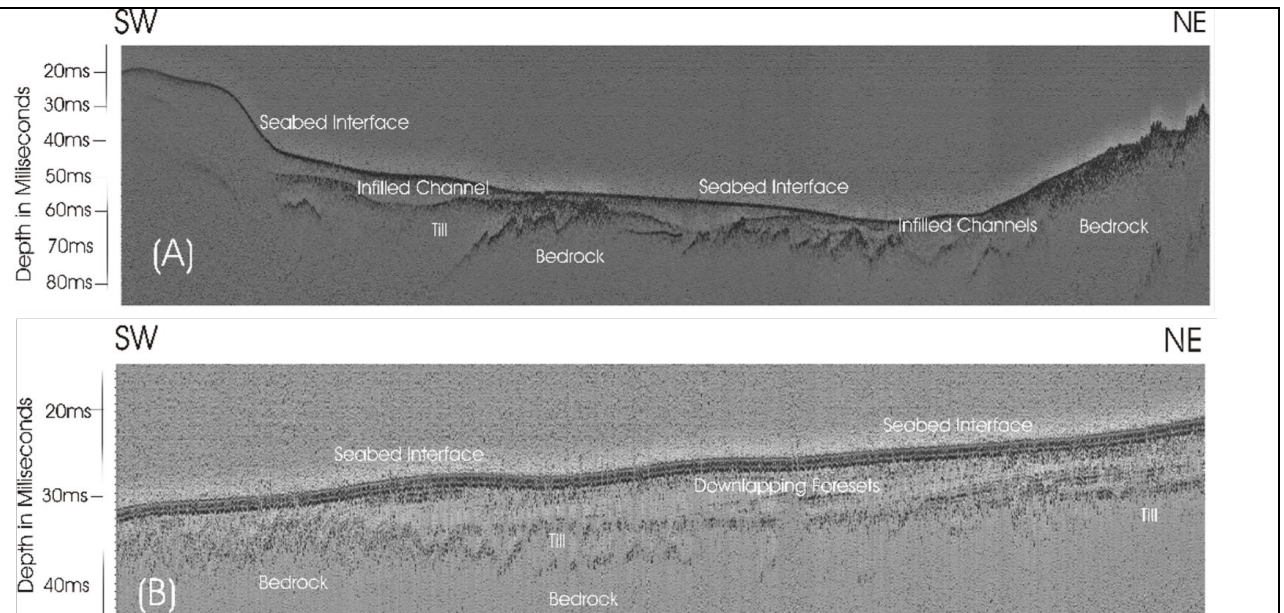
Fig. 7 – Examples of seismic pinger (3.5kHz) data. (A) Infilled palaeochannels visible across the outer bay area; (B) Prograding palaeodelta is visible extending southwest from the present day inner bay area. Position of lines is shown in Fig. 1.
