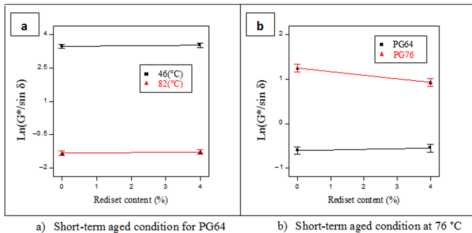
Fig. 7. Interaction effects of Rediset with temperature and binder type on the value of \text{Ln}(G^*/\sin \delta) for selected conditions
