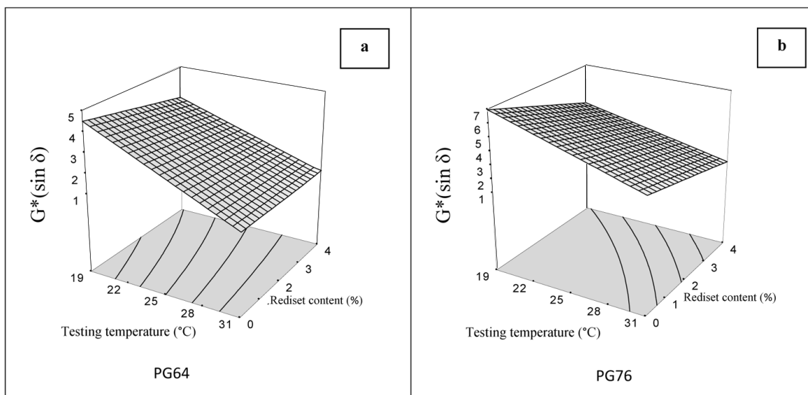
Fig. 9. Plot of response surface for G^*(\sin \delta) values for long-term aging conditions
