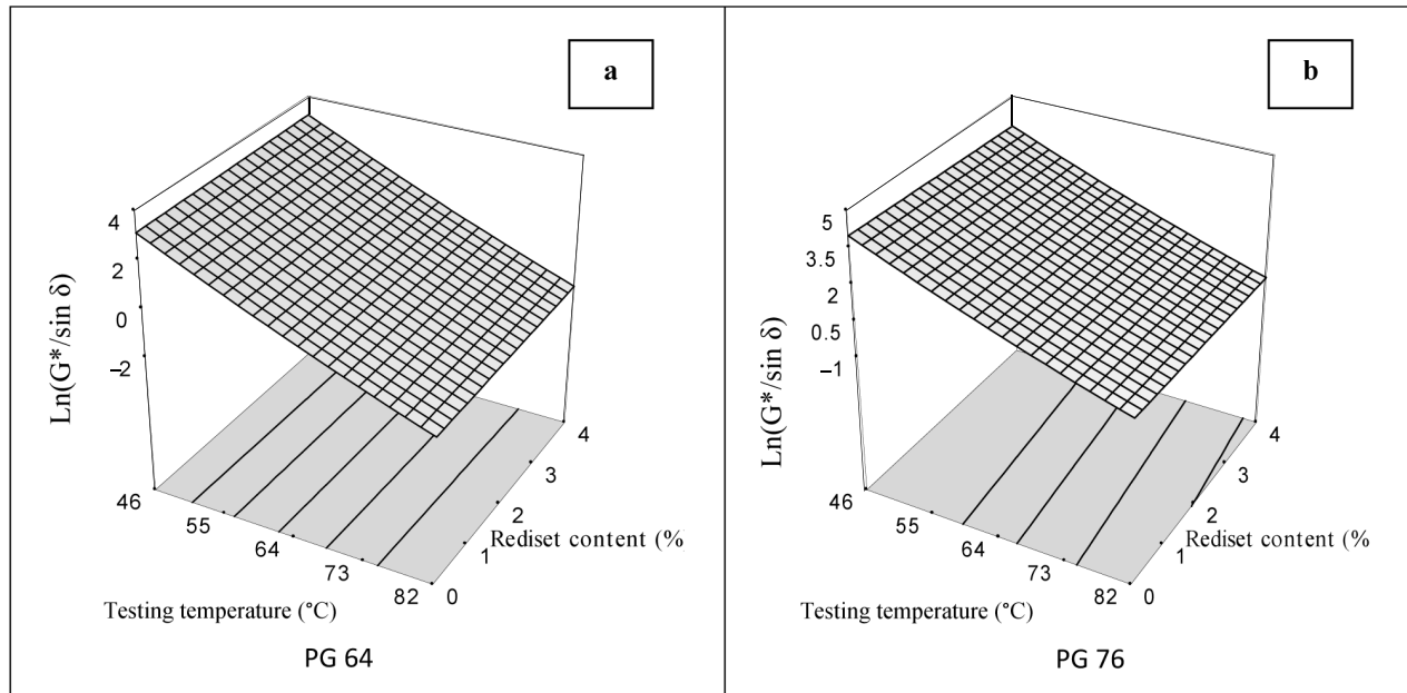
Fig. 6. Plot of response surface for the \text{Ln}(G^*/\sin \delta) value for unaged conditions
