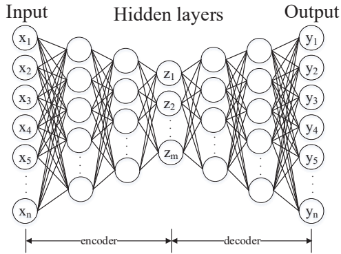
Fig. 2: Structure of deep autoencoder
