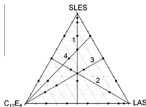
Fig. 3. Ternary C 12 E 8 /LAS/SLES diagram, showing the points at which SANS measurements were made; where line 1 represents equal C 12 E 8 and LAS mole fractions, line 2 equal C 12 E 8 and SLES mole fractions, line 3 equal SLES and LAS mole fractions, line 4 differing C 12 E 8 , LAS and SLES mole fractions, and the edges of the triangle the binary mixtures.
