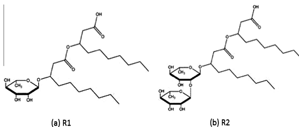
Fig. 1. Structure of the rhamnolipids R1, and R2.
