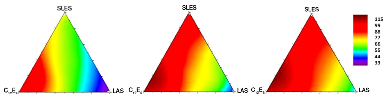
Fig. 4. Variation in aggregation number with solution composition, at (a) 10 mM, (b) 25 mM and (c) 50 mM. The legend indicates the colour scale which ranges from 33 (purple) to 115 (red).
