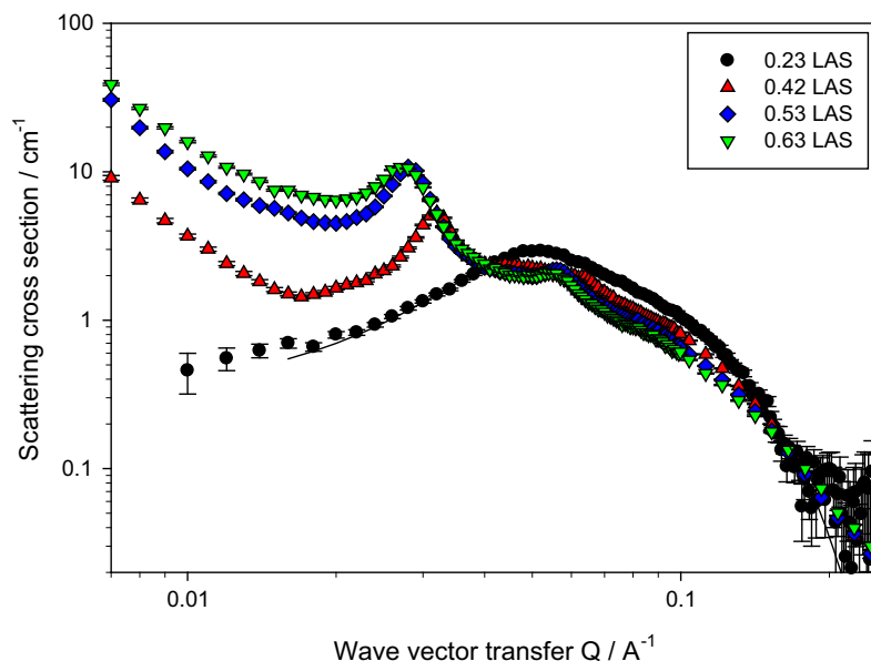
Fig. 7. SANS data for 50 mM R1/R2/C 12 E 8 /LAS/SLES with 30/70 mol ratio R/C (rhamnolipid/conventional surfactant ratio), and R1/R2 1:1 mol ratio. See legend for details. The R1, R2 mol ratios are 0.15, 0.15, and the C 12 E 8 and SLES mole fractions are 0.24, 0.14, 0.08, and 0.035 respectively. The solid line for the micellar scattering is a model calculation as described in the main text.
