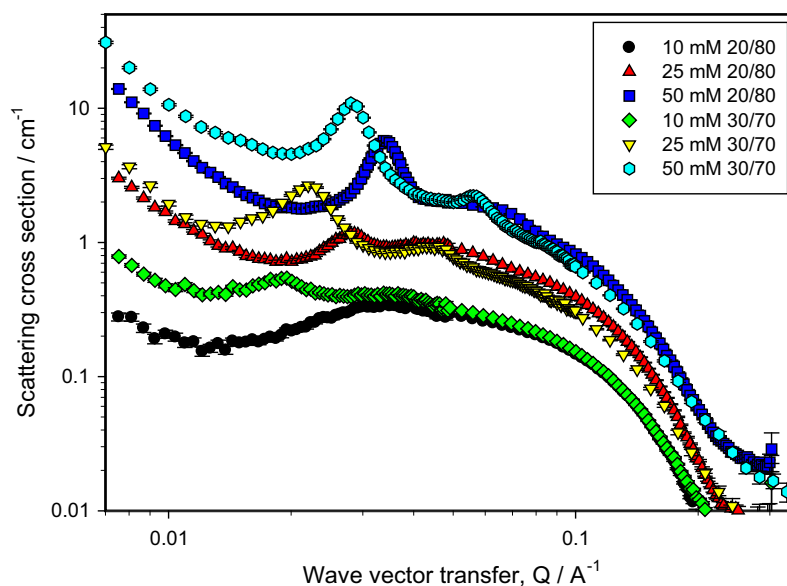
Fig. 8. SANS data for R1/R2/C 12 E 8 /LAS/SLES at 20/80 and 30/70 rhamnolipid/surfactant, at a fixed R1/R2 ratio of 2:1, at an equivalent C 12 E 8 /LAS/SLES solution composition of 0.125/0.75/0.125, at 10, 25 and 50 mM, see legend for details.
