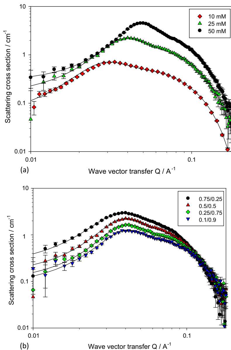
Fig. 2. SANS data for (a) 0.5/0.5 C_{12}E_8 /SLES at 10 mM, 25 mM and 50 mM, and (b) 25 mM C_{12}E_8 /SLES at compositions 0.75/0.25, 0.5/0.5, 0.25/0.75 and 0.1/0.9, at 25 mM. See legend for details. The solid lines are model calculations as described in the text and for the key model parameters summarised in Table 1, and in Table S1 in the Supporting Information.
