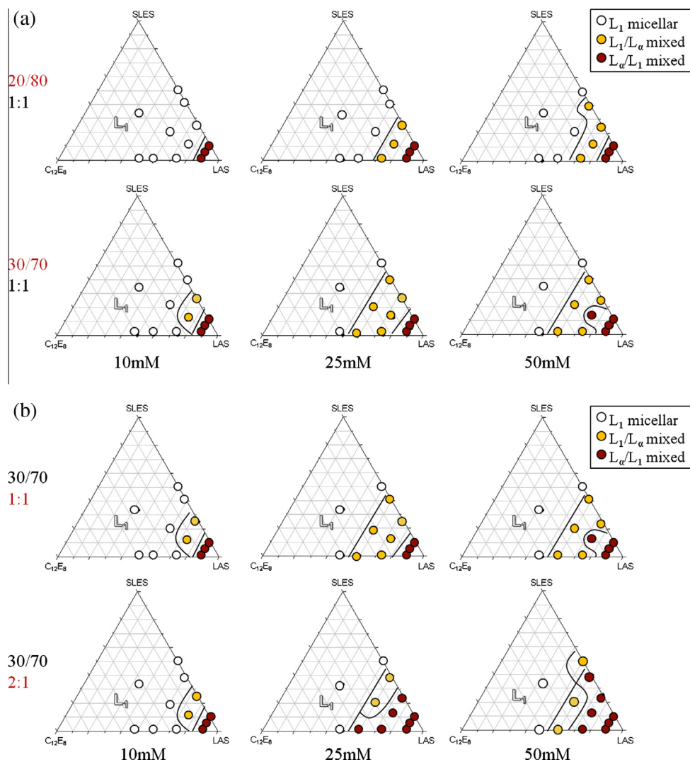
Fig. 9. Approximate qualitative phase diagrams for R1/R2/C 12 E 8 /LAS/SLES surfactant mixtures, derived from SANS data, at 10, 25 and 50 mM, (a) variation in rhamnolipid/surfactant mole ratio, (b) variation in R1/R2 mol ratio.
