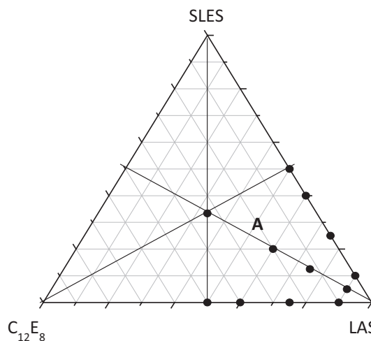
Fig. 6. Ternary diagram for C_{12}E_8 /LAS/SLES, showing compositions used for more detailed evaluation of the lamellar/micellar coexistence region.
