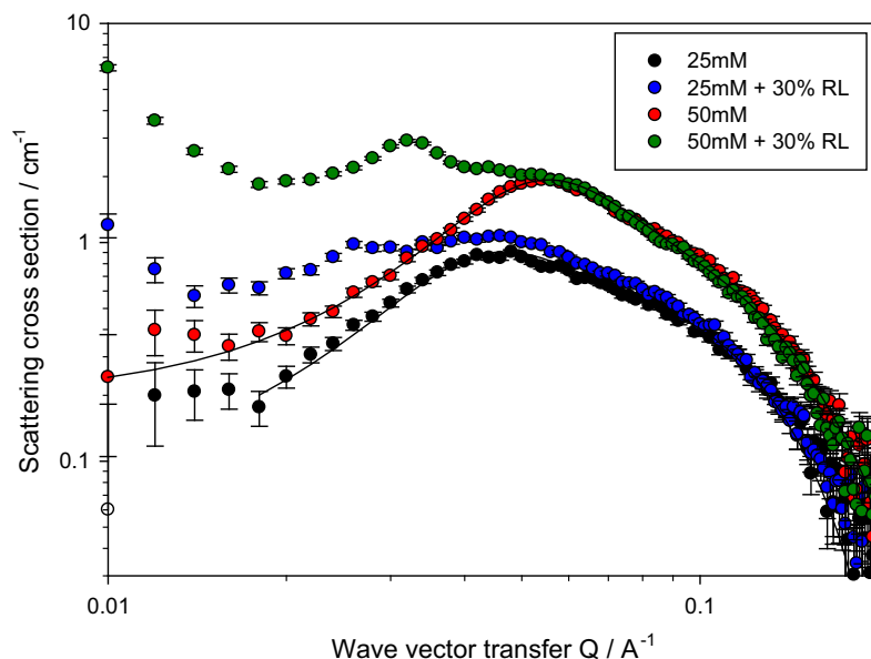
Fig. 5. SANS data for 0.125/0.75/0.125 mol ratio C_{12}E_8 /LAS/SLES at 25 and 50 mM, in the absence and presence of 30 mol% replacement by a 1:1 mol ratio mixture of R1/R2. See legend for details. The solid lines are model fits as described in the text.
