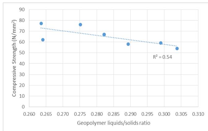
Figure 5. Effect of geopolymer liquids to geopolymer solids ratio on the 28 day compressive strength of geopolymer mortar.
