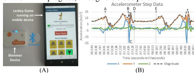
Figure 1. (A) Shows the Shimmer device and a mobile phone running the Leckey Game app. The Shimmer device connects to the mobile app via Bluetooth. (B) Shows accelerometer data of 2 walking steps of the left foot, of an un-impaired adult. A: toe off. A to B: foot swing. C: heel strike. D to E: Left foot stationary, right foot moving.
