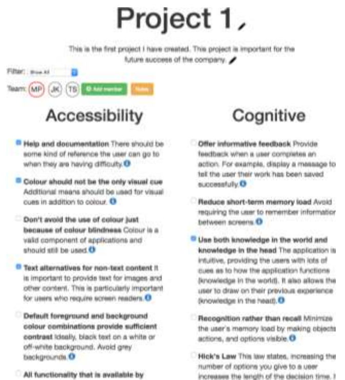
Figure 1. Partial screenshot of the interactive HCI tool.
