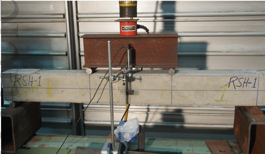
Figure 3: Experimental setup for four-point loading
