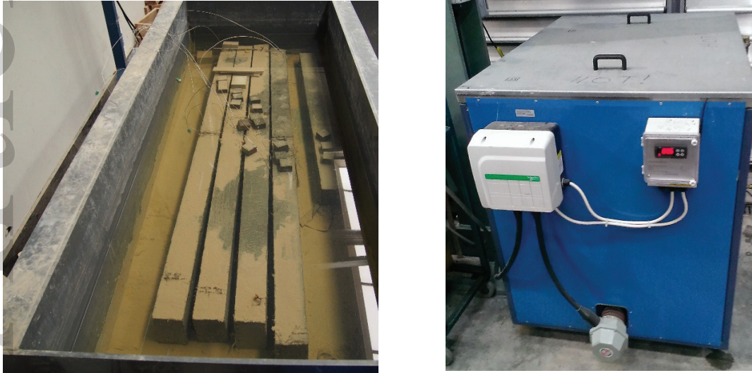
Figure 2. Left) cold curing tank, right) hot curing tank
