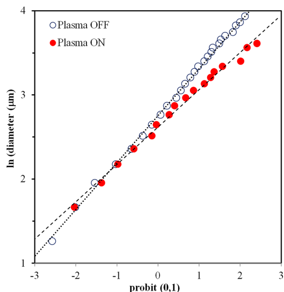
FIG. 3. Log-probability plot of \ln(D) in \mu\text{m} against the inverse standard normal distribution (probit) for droplet size distributions with and without plasma. The dotted lines in each case are least-square linear fits with R^2 values >0.99 .
