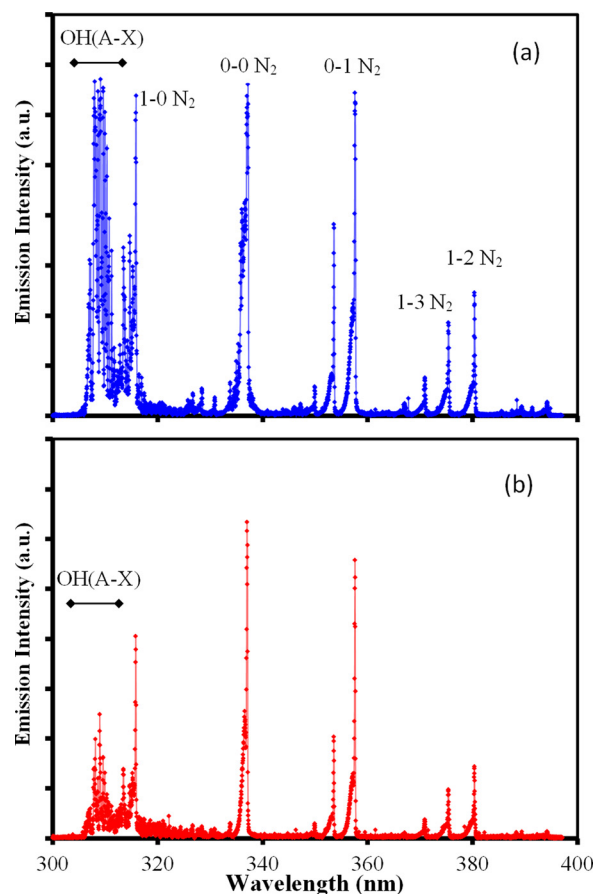
FIG. 5. Optical emission spectra indicating \text{N}_2 and OH(A-X) emission lines for (a) plasma—no aerosol and (b) plasma with aerosol.
