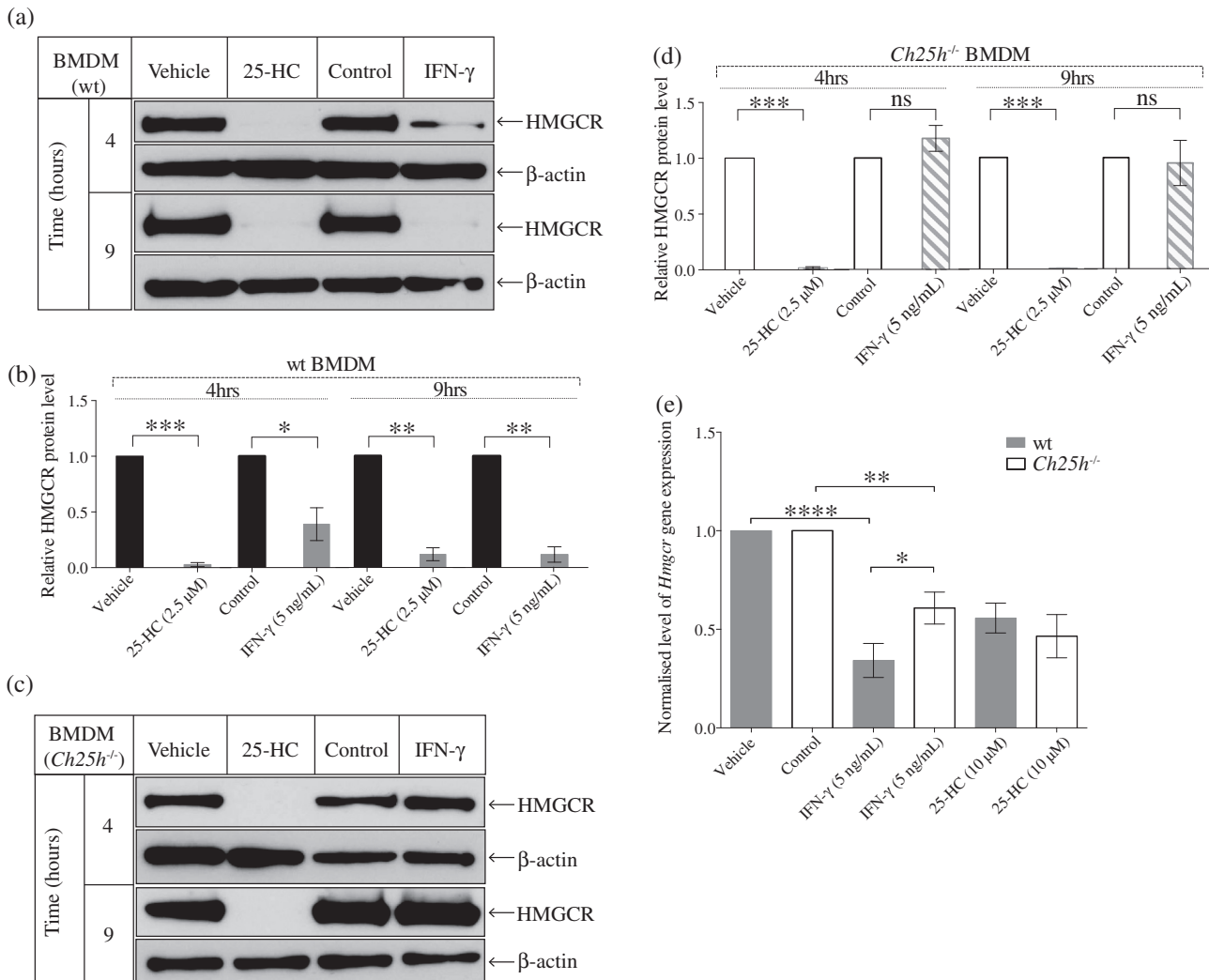
Fig. 5. Comparison of Hmgcr mRNA and HMGCR protein levels following 25-HC or IFN- \gamma treatment in wild-type and Ch25h -/- BMDMs. (a) Western blot analysis of HMGCR with 2.5 \mu M of 25-HC or 5 ng/mL of IFN- \gamma treatment in Medium C at 4-h and 9-h time points in wild-type BMDMs. (b) Intensity values of HMGCR to \beta -actin. Bars present the mean \pm SEM ( n = 3 ). (c) Western blot analysis of HMGCR with 2.5 \mu M of 25-HC or 5 ng/mL of IFN- \gamma treatment in Medium C at 4-h and 9-h time points in Ch25h -/- BMDMs. (d) Intensity values of HMGCR to \beta -actin. Bars present the mean \pm SEM ( n = 3 ). (e) HMGCR transcript abundance in wild-type and Ch25h -/- BMDMs with 2.5 \mu M of 25-HC or 5 ng/mL of IFN- \gamma treatment for 24 h in Medium A. The 25-HC-treated groups were normalised by the Vehicle and the IFN- \gamma -treated groups were normalised by the control treated samples, respectively. Bars present the mean \pm SEM ( n = 9 ). * p < 0.05 , ** p < 0.01 , *** p < 0.001 , determined with an unpaired Student's t test.
