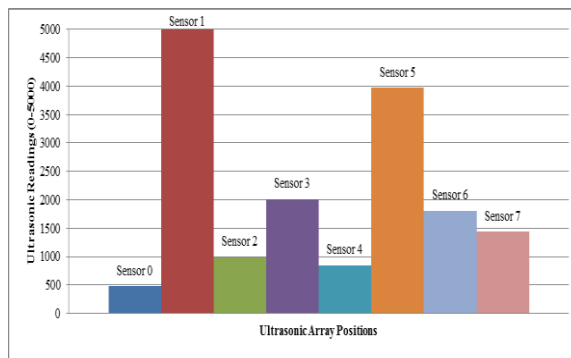
Figure 5. Ultrasonic array sensor data for the determination of the door-closed state.
