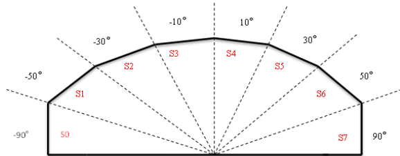
Figure 1. The arrangement of the ultrasonic sensors in the array.
