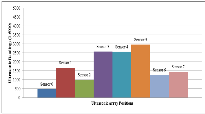
Figure 6. Ultrasonic array sensor data for the determination of the door-opened state.
