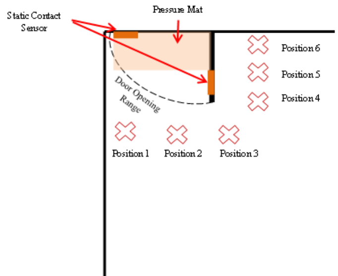
Figure 3. The six robot placement positions in the door region utilized within each of the three experimental stages of this study. The placements of the pressure mat and contact sensor are also depicted.
