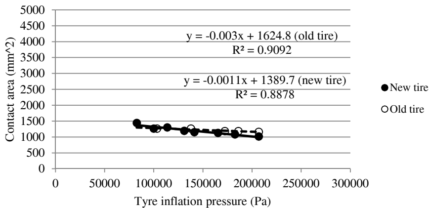
Figure 4. Contact area v. tyre inflation pressure – excluding lower and higher inflation data
