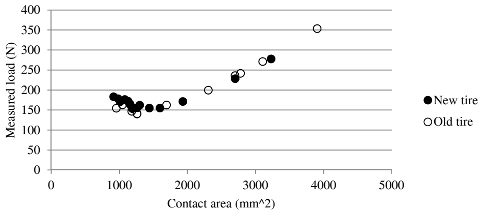
Figure 7. Measured load v. contact area – all data
