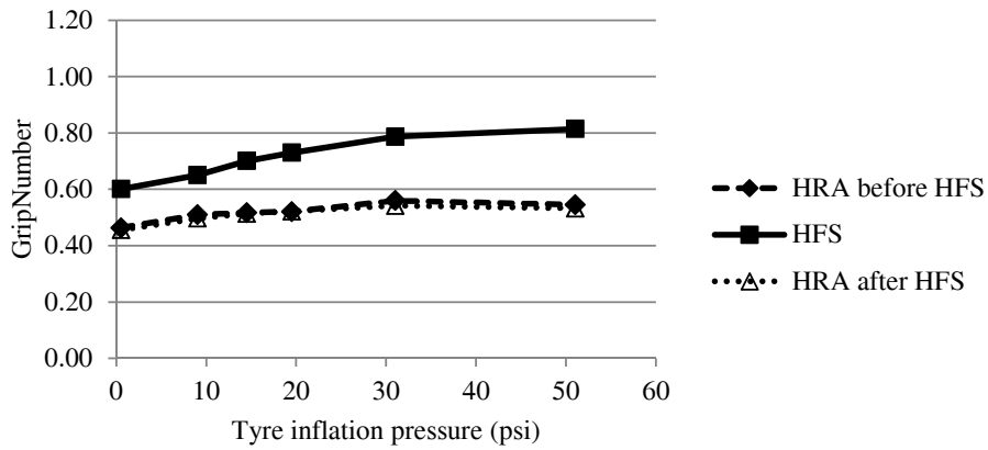
Figure 12. GripTester data for worn tyre
